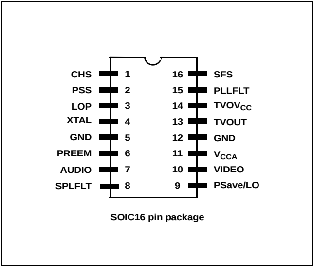
Figure 1. Pin Connections
