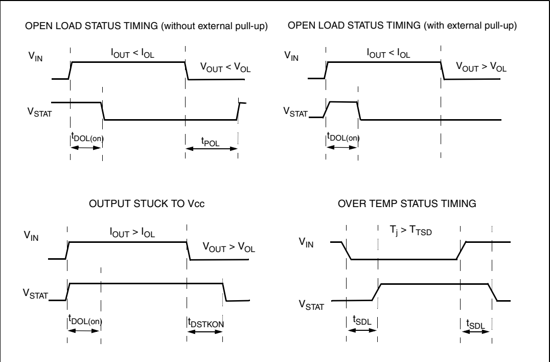
Figure 4. Status timings
