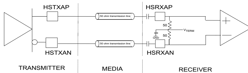
Figure 7-3. Example of High Speed I/O AC Coupled Mode
