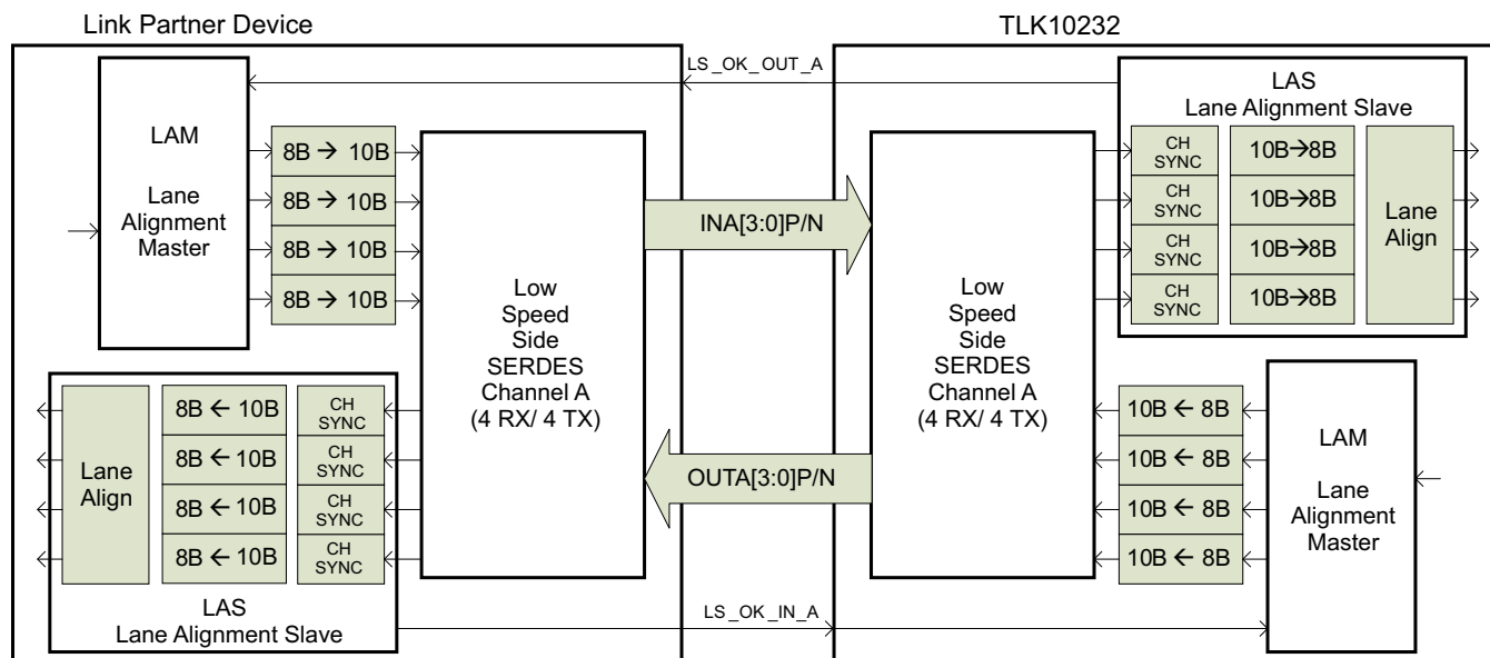
Figure 5-2. Block Diagram of the Lane Alignment Scheme
