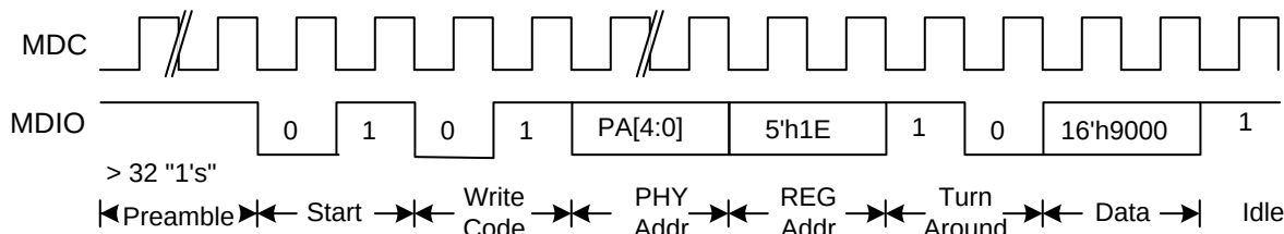
Figure 7-13. CL22 - Indirect Address Method – Address Write
