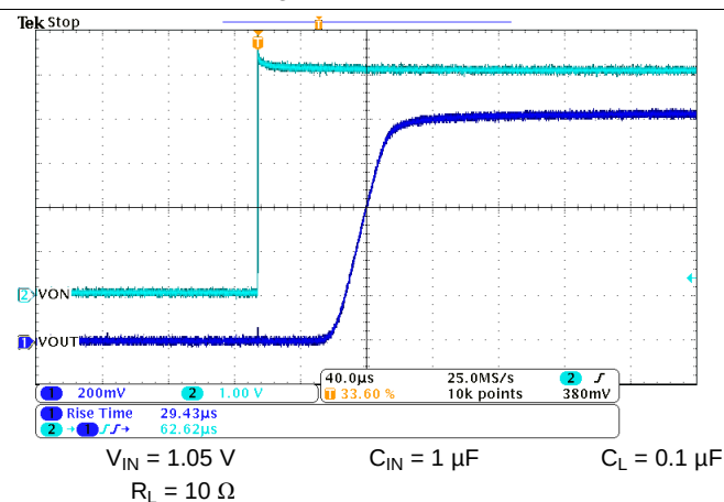
Figure 20. t_R at V_{IN} = 1.05 V
