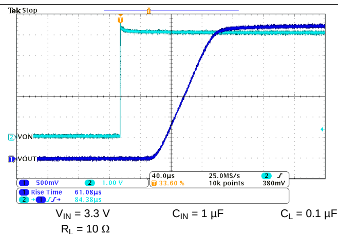
Figure 18. t_R at V_{IN} = 3.3 V
