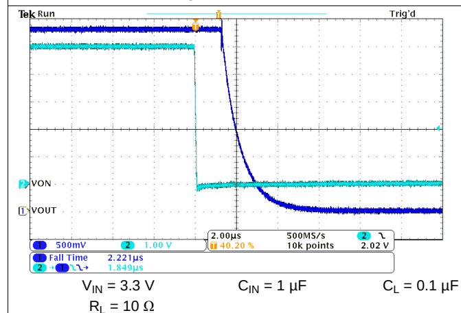
Figure 19. t_F at V_{IN} = 3.3 V
