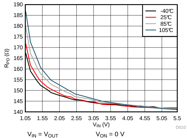
Figure 10. R_{PD} vs V_{IN}
