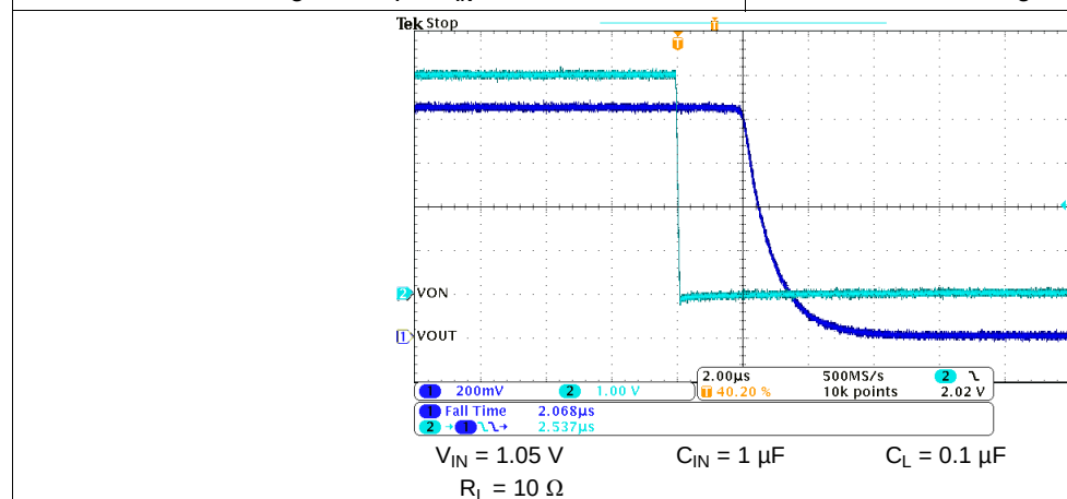
Figure 21. t_F at V_{IN} = 1.05 V
