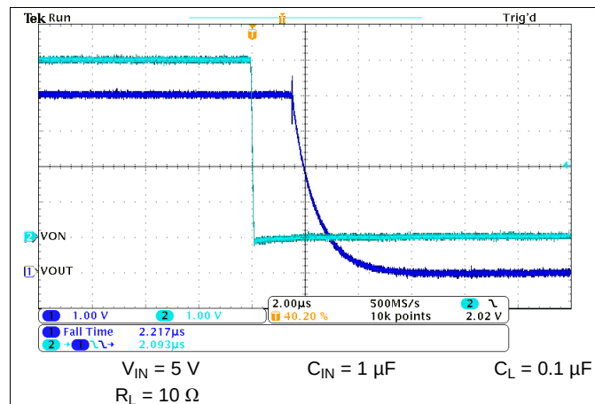
Figure 17. t_F at V_{IN} = 5 V
