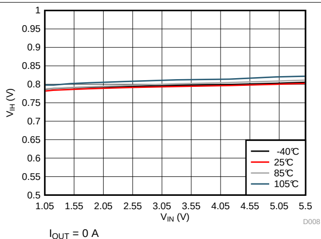
Figure 8. V_{IH} vs V_{IN}
