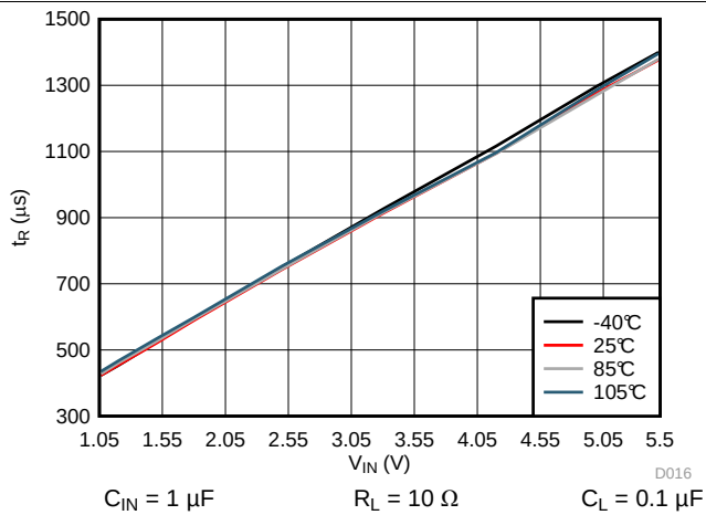
Figure 22. t_R vs V_{IN}
