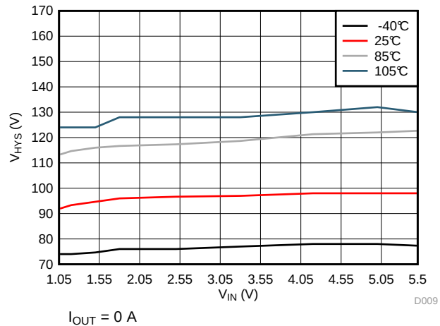
Figure 9. V_{HYS} vs V_{IN}
