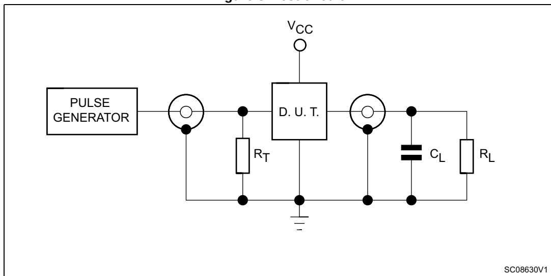
Figure 8. Test circuit
