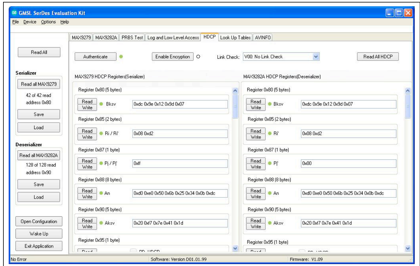
Figure 8. MAXSerDesEV-D Evaluation Kit Software (HDPC Tab)
