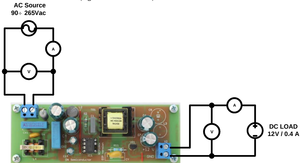
Figure 1: Test Setup for Flyback Converter
