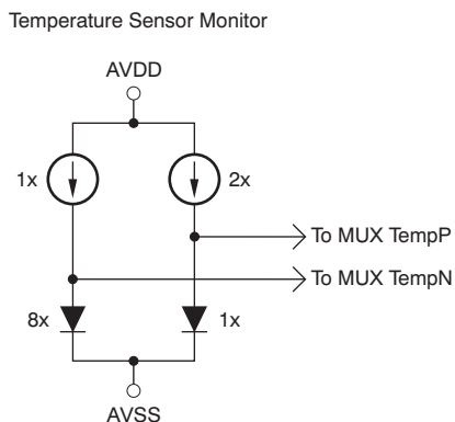
Figure 16. Measurement of the Temperature Sensor in the Input
