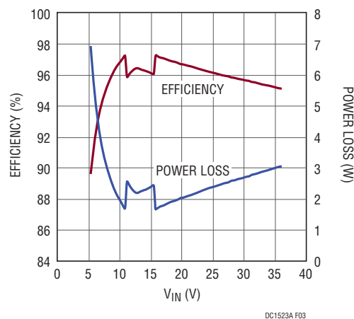
Figure 3. Efficiency and Power Loss at Full Load. The Power Loss is Highest in Boost Mode Due to the High Inductor Current, and Drops as Input Voltage Increases. Switching Losses Again Increase when V_{IN} > V_{OUT} . All Four MOSFETs are Switching in Buck-Boost Mode and This Shows Up as a Small Increase in Losses When V_{IN} = 11V to 15.5V
