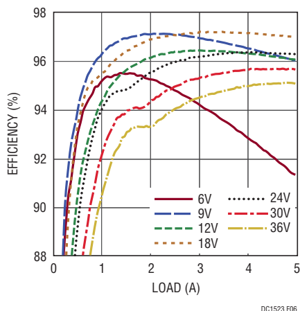
Figure 6. Efficiency at Various Input Voltages
