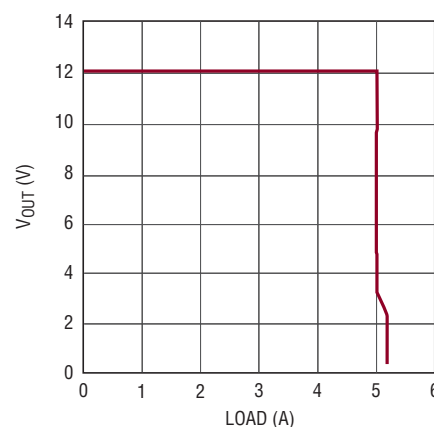
Figure 7. Output Current Limit. ( V_{IN} = 12V . The Easiest Way to Do This Test is with an Active Load in Voltage Mode)
