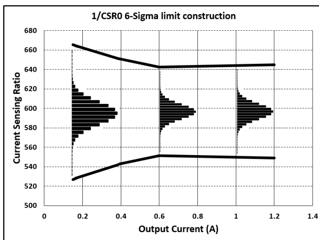
Figure 20. CSR0 limit construction versus population of devices
