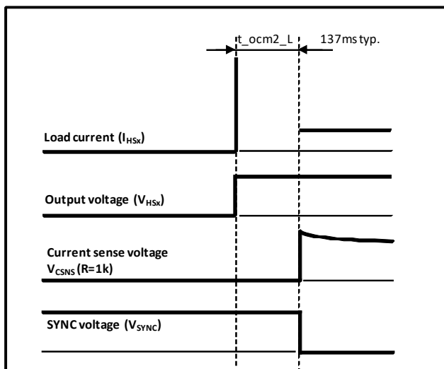
Figure 15. Current sense blanking during overcurrent window activity
