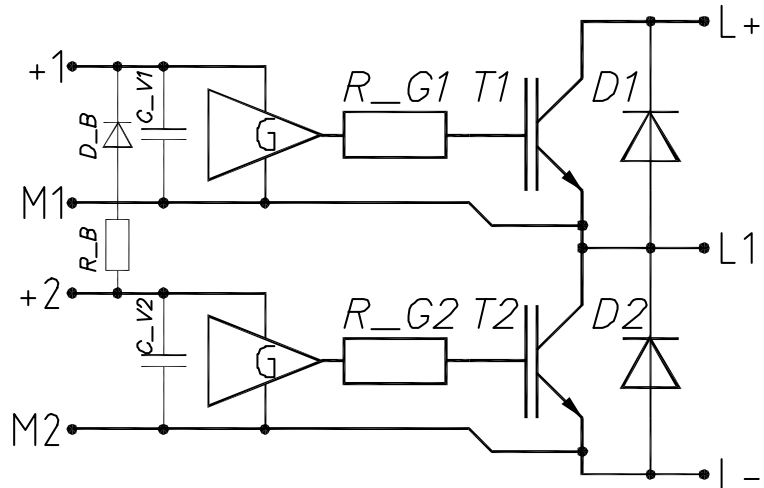
Fig. 2 Bootstrap circuit
