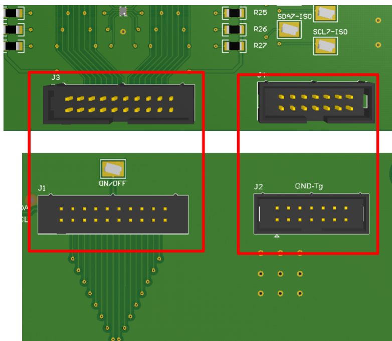
Figure 16. Ribbon Wire Headers on Both Boards (Top = Programming Board, Bottom = Socket Board)
