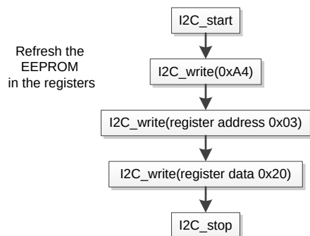
Figure 5. I 2 C Command Chain for Refreshing the Registers
