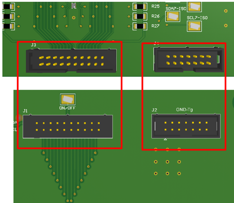
Figure 40. Ribbon Wire Headers on Both Boards (Top = Programming Board, Bottom = Socket Board)
