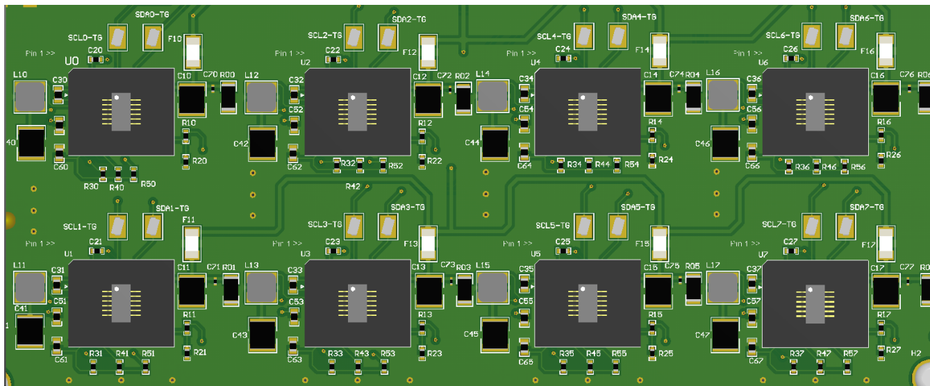
Figure 24. Sockets With Device Populated in Proper Orientation
