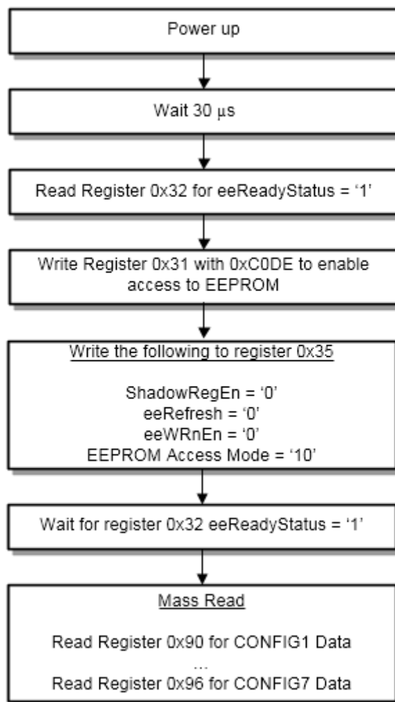
Figure 9. DRV10983-Q1 and DRV10987 Mass Read Protocol Using I 2 C
