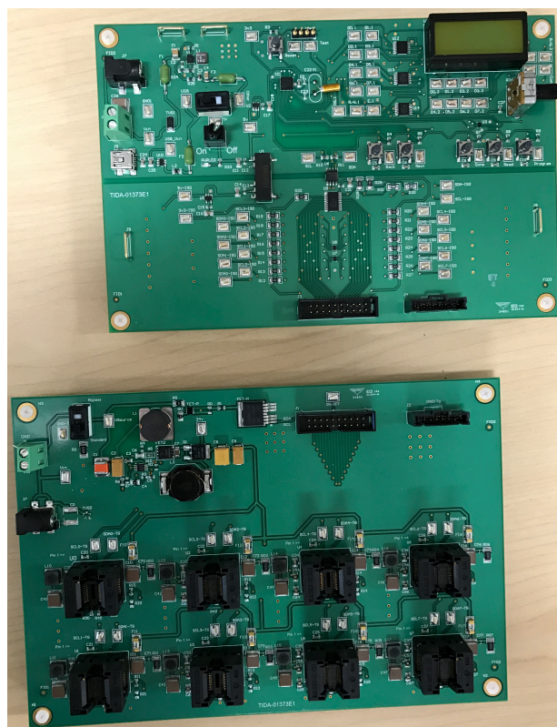
Figure 11. TIDA-01373 Board Image
