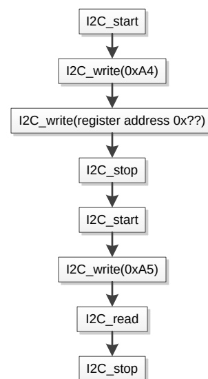
Figure 6. I 2 C Command Chain for Reading a Register
