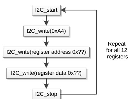
Figure 2. I 2 C Command Chain for Setting a Register
