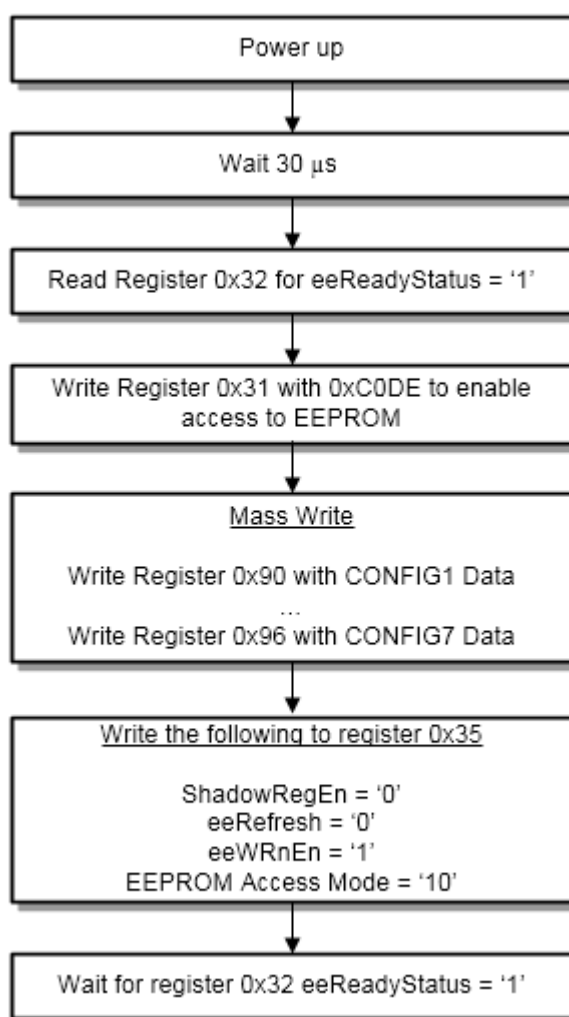
Figure 8. DRV10983-Q1 and DRV10987 Mass Write Protocol Using I 2 C
