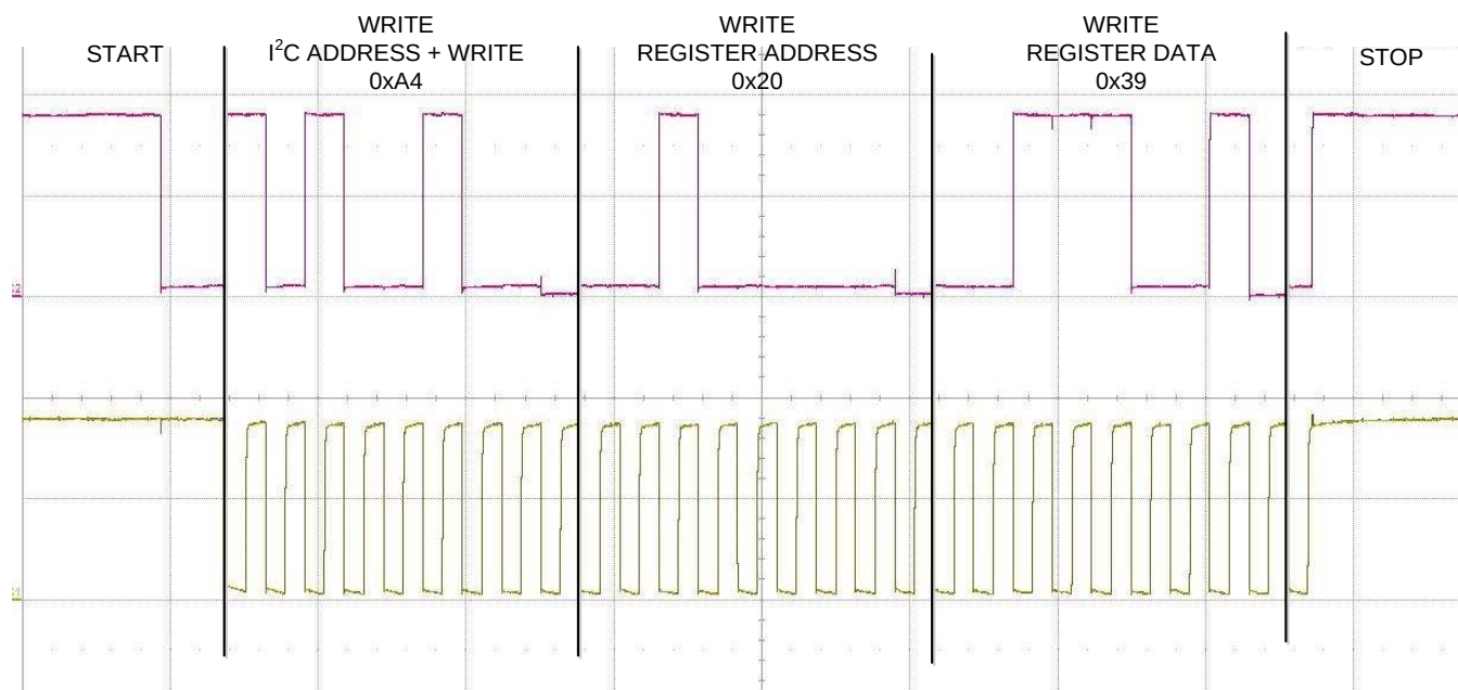
Figure 3. I 2 C Waveform of Writing to a Register
