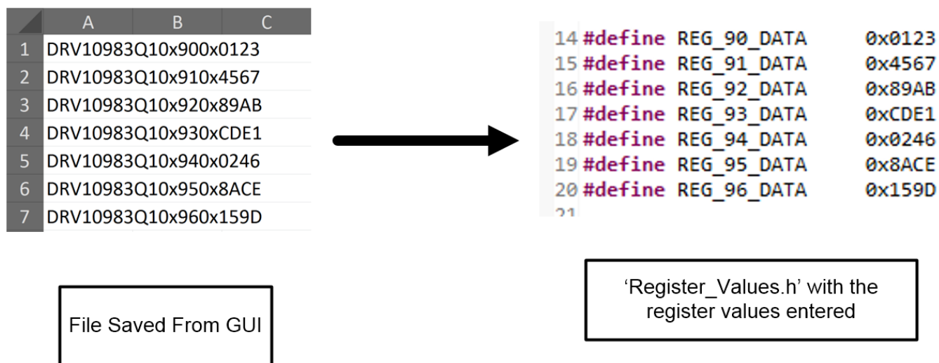
Figure 42. Example Register Settings Entered Into the Programming Tools Code for DRV10983-Q1
