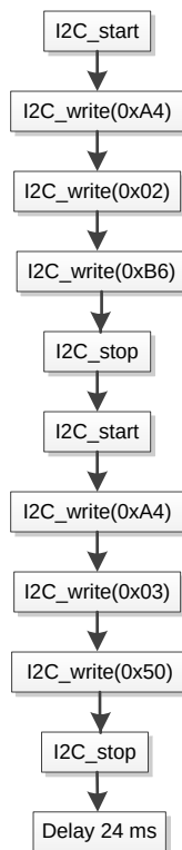
Figure 4. I 2 C Command Chain for Writing to EEPROM
