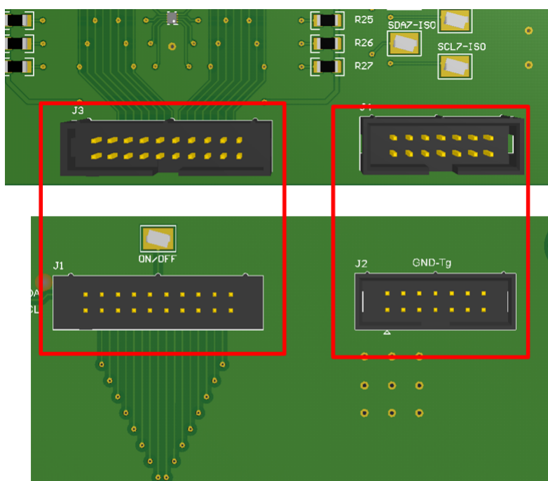
Figure 23. Ribbon Wire Headers on Both Boards
