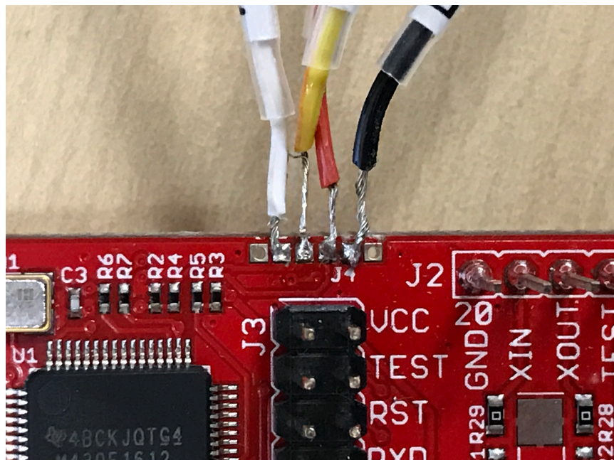
Figure 60. LaunchPad™ 4-Pin Programming Header with Soldered Wires
