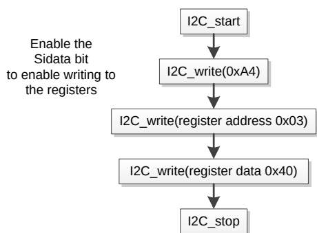
Figure 1. I 2 C Command Chain for Enabling Sidata Bit
