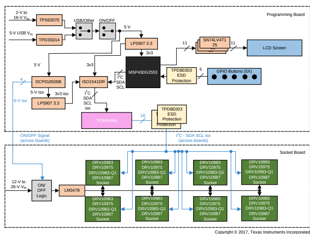
Figure 10. TIDA-0137 Block Diagram
