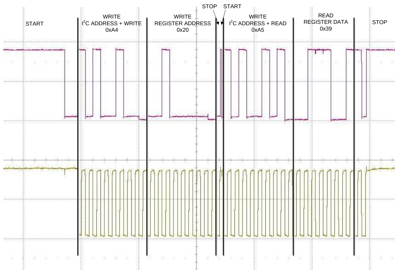
Figure 7. I 2 C Waveform of Reading a Register
