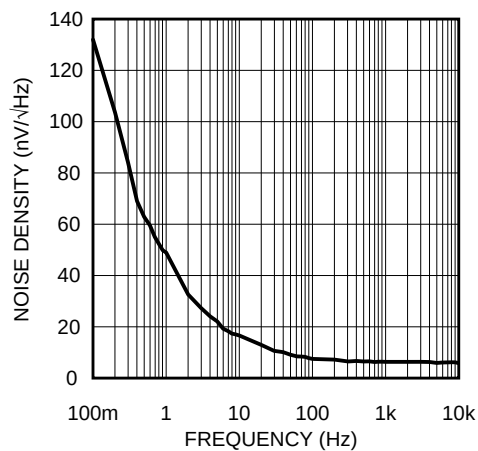
Figure 30. Input-Referred Noise Density vs. Frequency
