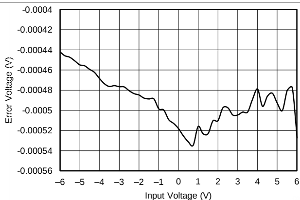
Figure 31. OPA317 Output Voltage vs Input Voltage
