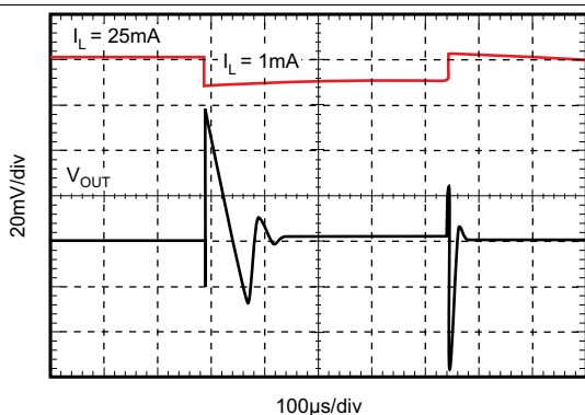
Figure 19. 1 to 25-mA Load Transient ( C_L = 1 \mu F )
