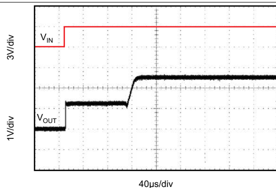
Figure 13. Step Response, C_L = 0 , 3-V Start-Up
