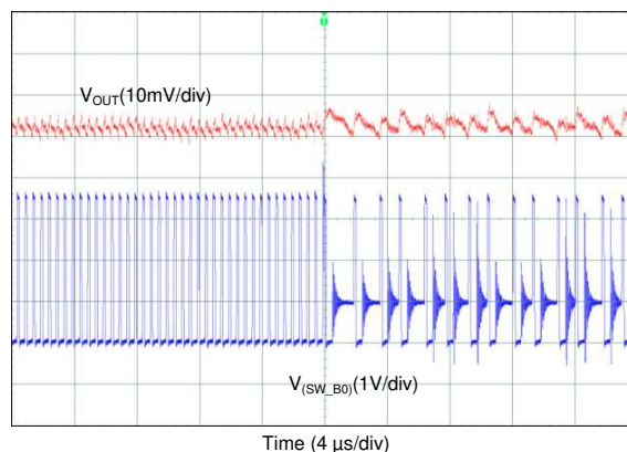
Figure 89. Transient from PWM-to-PFM Mode (4-Phase Output)
