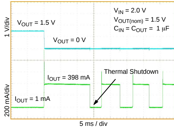
Figure 67. Short-Circuit Response V_{OUT} = 1.5\text{ V} , C_{OUT} = 1\text{ }\mu\text{F}
