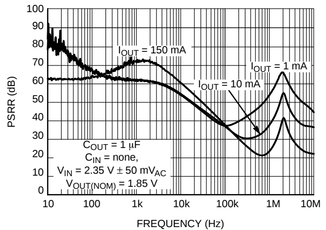
Figure 44. PSRR vs. Frequency V_{OUT} = 1.85 \text{ V}
