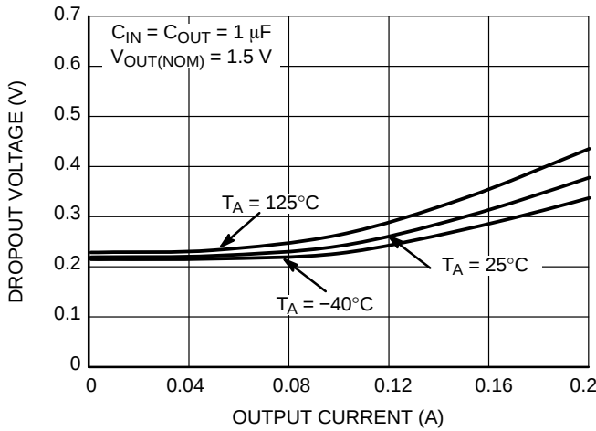
Figure 21. Dropout Voltage vs. Output Current V_{OUT} = 1.5\text{ V}
