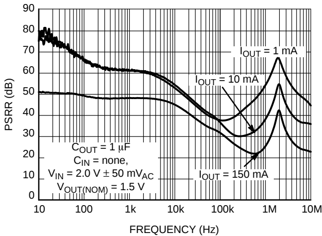
Figure 43. PSRR vs. Frequency V_{OUT} = 1.5 \text{ V}
