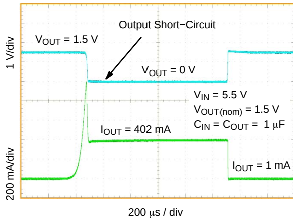
Figure 65. Short-Circuit Response V_{OUT} = 1.5\text{ V} , C_{OUT} = 1\text{ }\mu\text{F}
