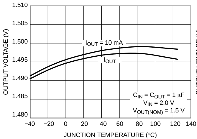
Figure 3. Output Voltage vs. Temperature V OUT = 1.5 V
