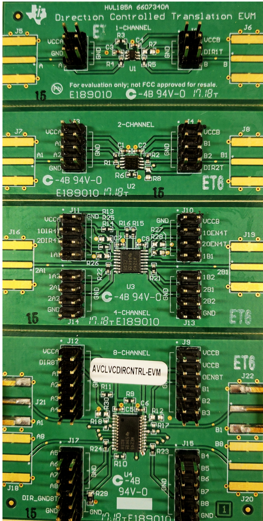
Figure 1. SN74XVCXTX45EVM: 8, 4, 2, 1 Channel versions
