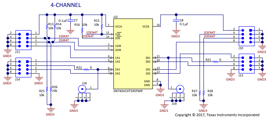
Figure 6. Four Channel
