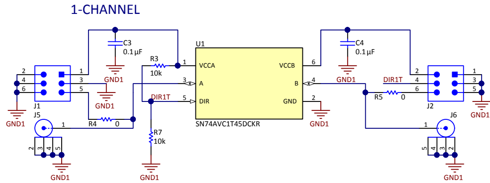
Figure 4. One Channel
