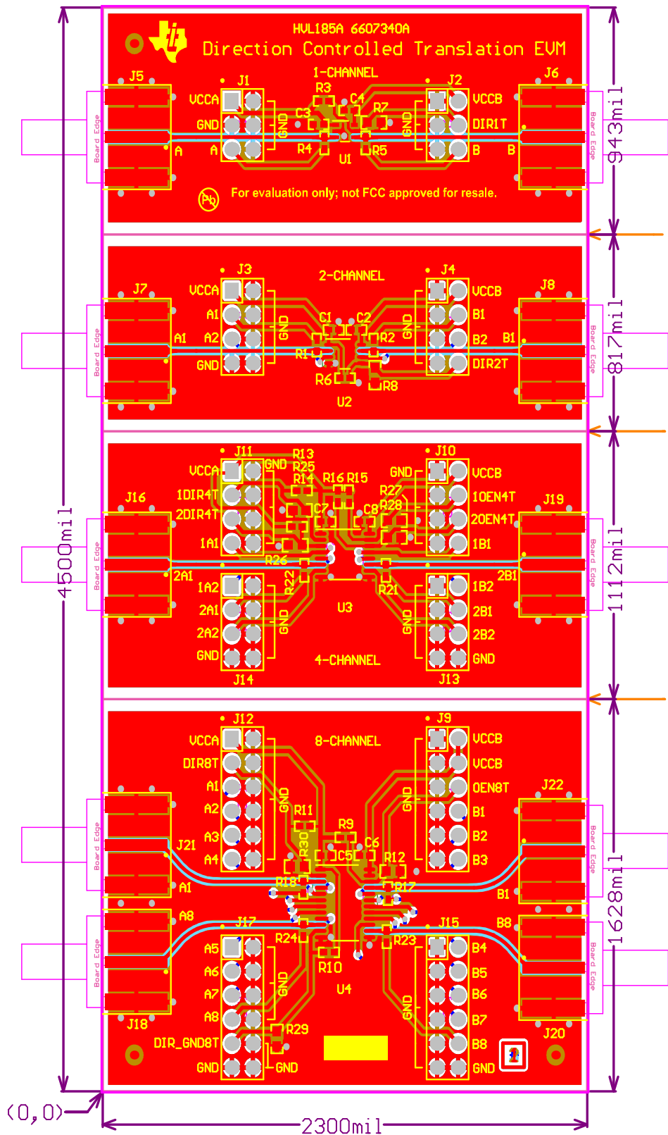
Figure 2. AVCLVCDIRCNTRL-EVM Layout
