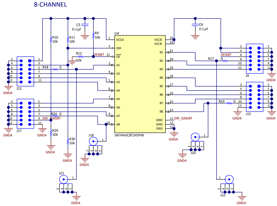
Figure 7. Eight Channel
