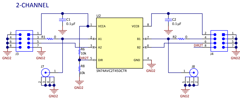
Figure 5. Two Channel
