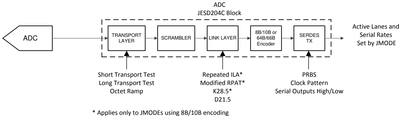
Figure 28. Test Mode Insertion Points
