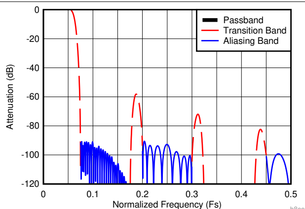
Figure 16. Decimate-by-8 Composite Response
