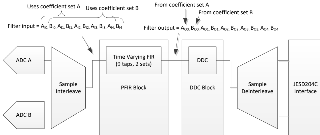
Figure 9. Time Varying Filter PFIR Block Diagram
