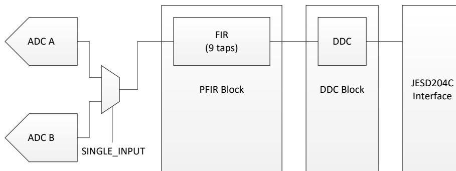
Figure 8. Single Channel Equalization PFIR Block Diagram
