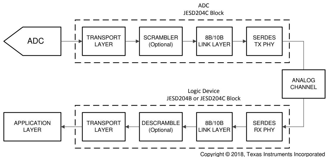
Figure 22. Simplified 8B/10B Encoded JESD204C Interface Diagram
