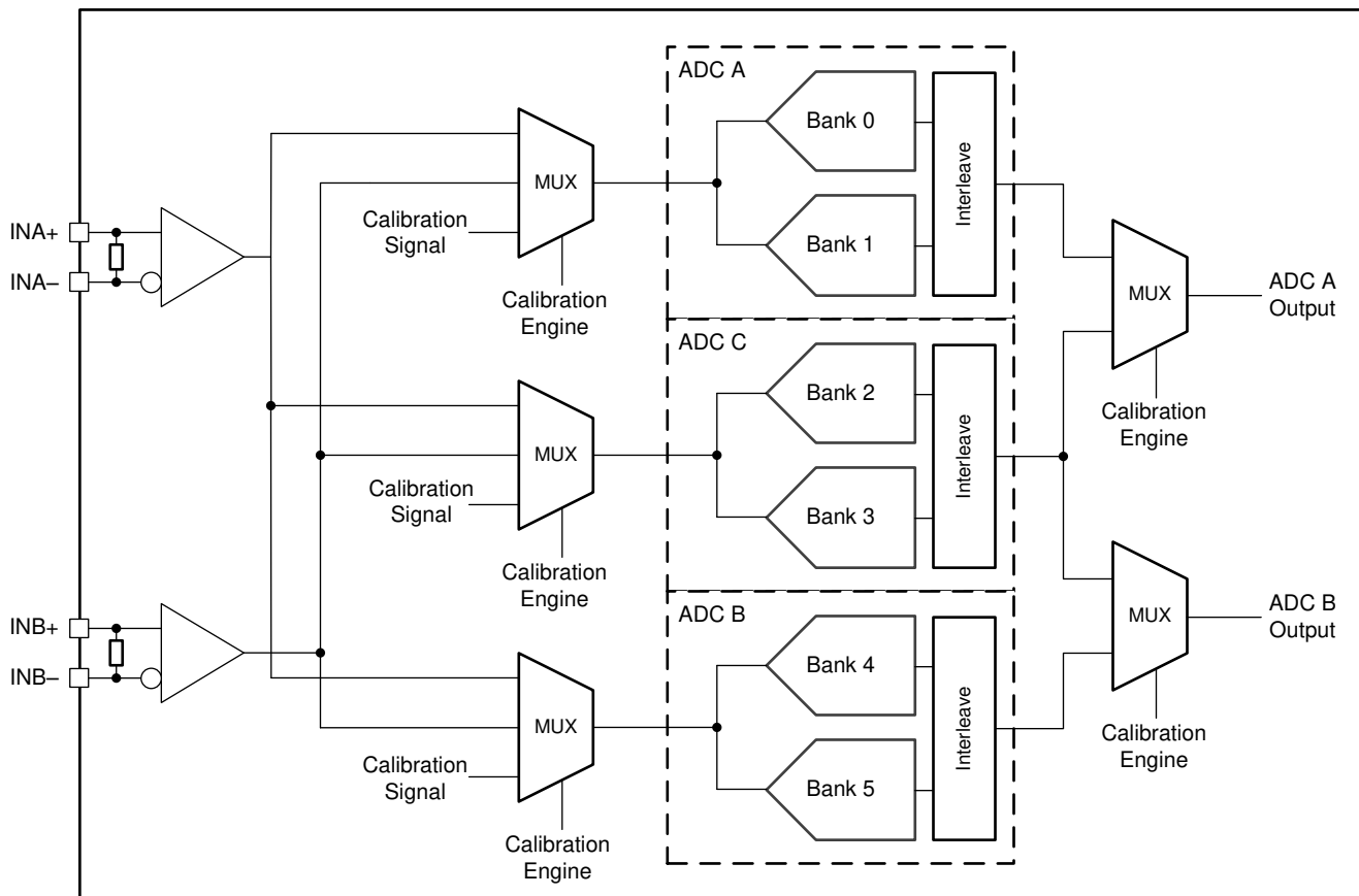
Figure 29. ADC12DJ5200RF Calibration System Block Diagram
