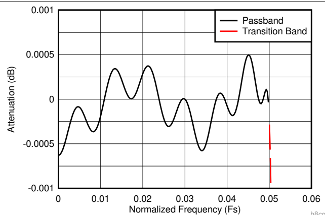
Figure 17. Decimate-by-8 Composite Zoomed Pass-Band Response
