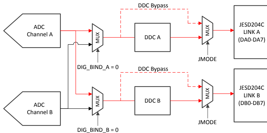
Figure 27. Dual DDC Mode or Redundant Data Mode for Channel A
