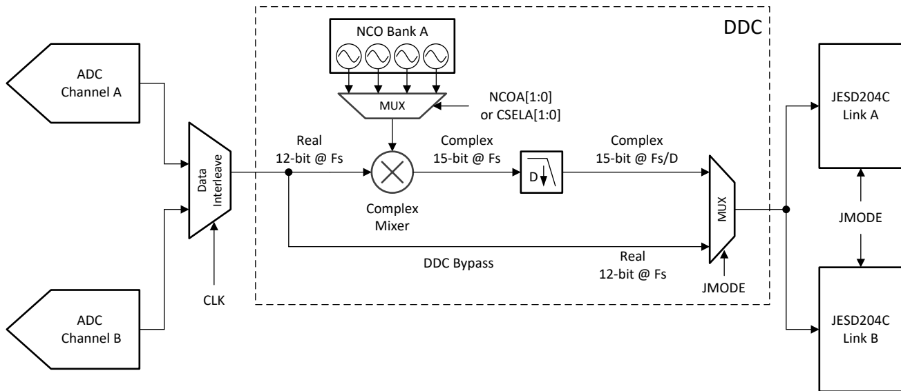
Figure 12. Digital Down Conversion Block in Single Channel Mode
