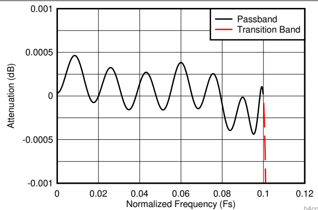
Figure 15. Decimate-by-4 Composite Zoomed Pass-Band Response
