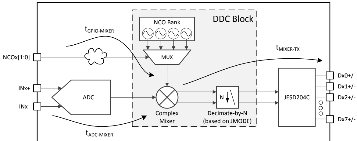
Figure 13. NCO Fast Frequency Hopping Latency Diagram
