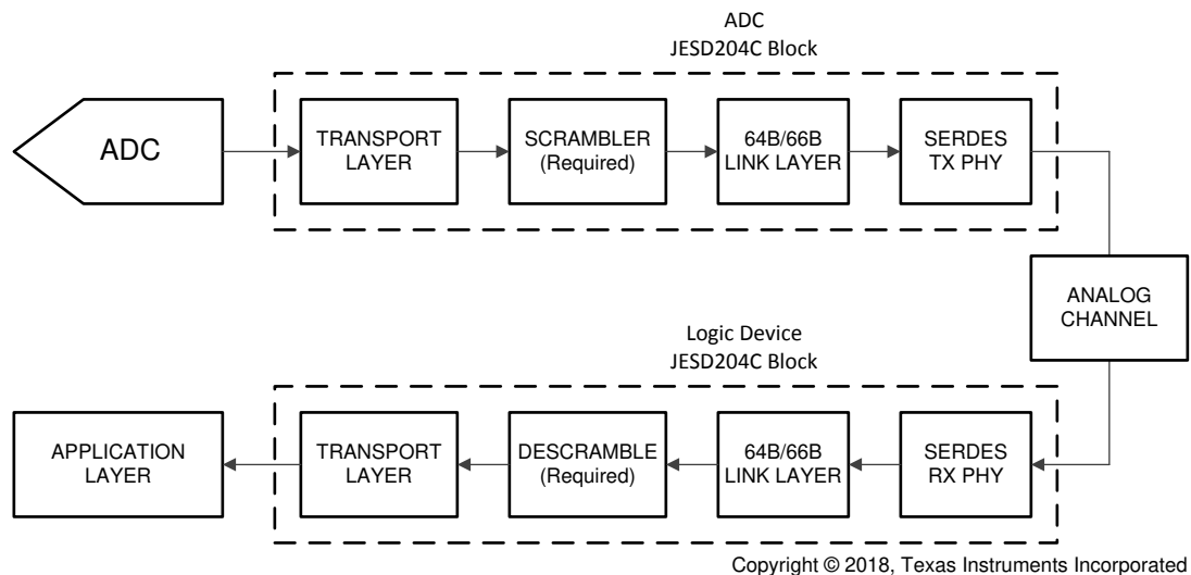
Figure 23. Simplified 64B/66B Encoded JESD204C Interface Diagram
