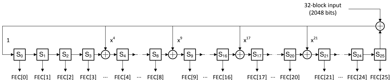
Figure 25. FEC Parity Bit Generator
