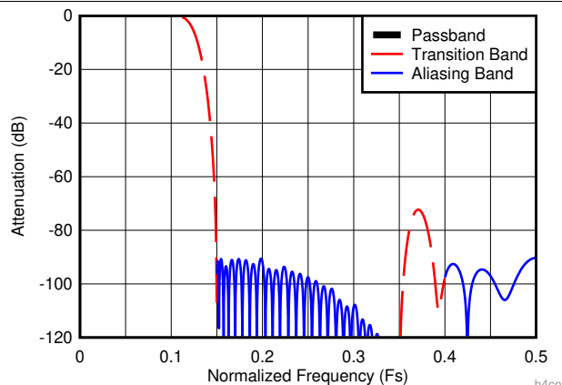
Figure 14. Decimate-by-4 Composite Response
