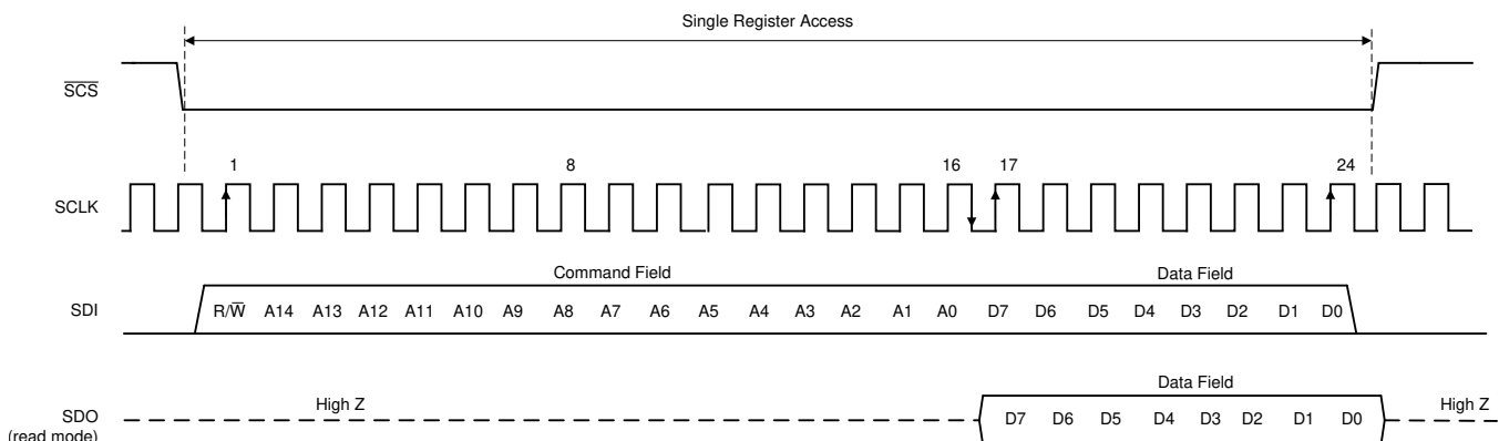
Figure 30. Serial Interface Protocol: Single Read/Write
