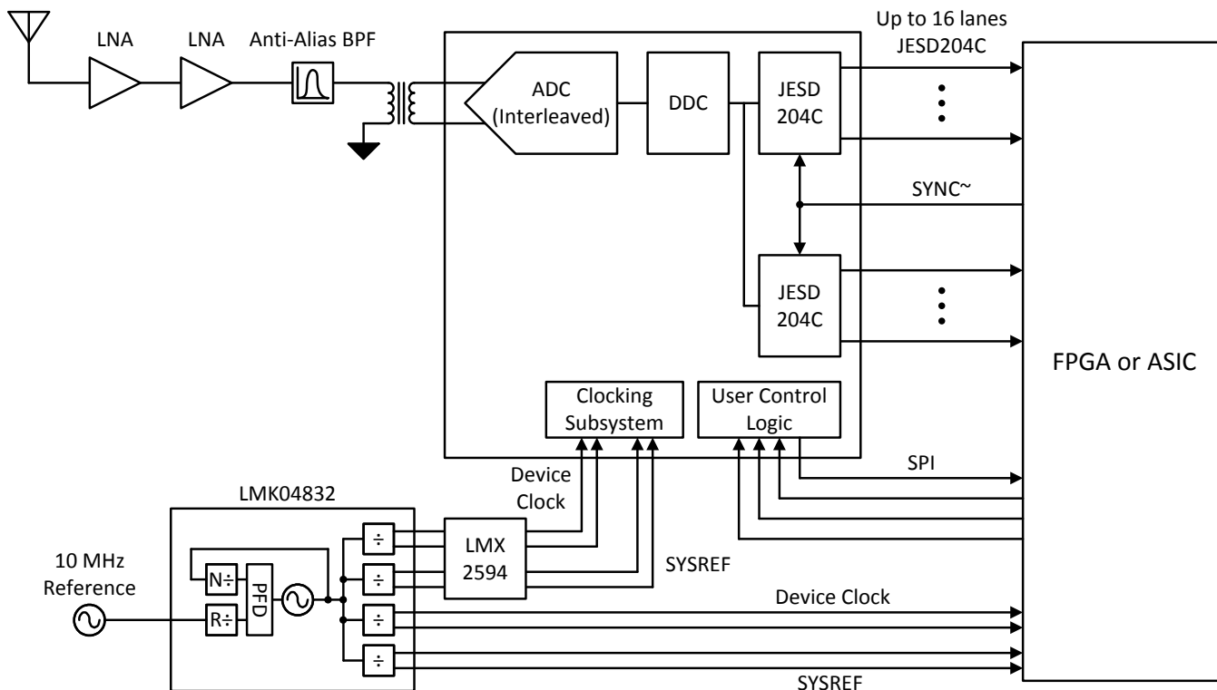
Figure 156. Typical Configuration for Wideband RF Sampling
