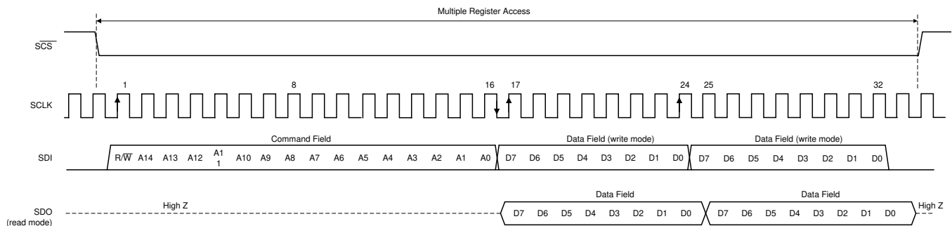
Figure 31. Serial Interface Protocol: Streaming Read/Write
