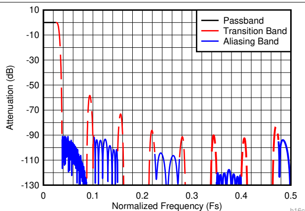
Figure 18. Decimate-by-16 Composite Response
