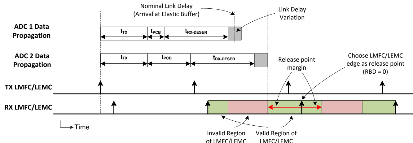
Figure 26. LMFC/LEMC Valid Region Definition for Elastic Buffer Release Point Selection
