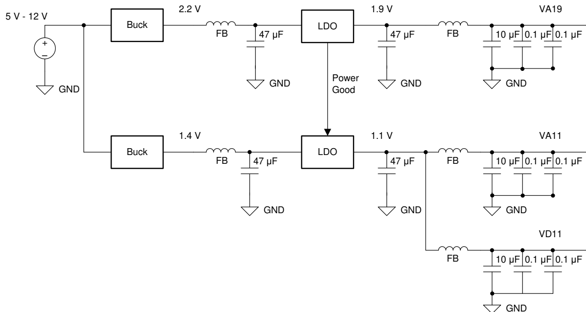
Figure 158. LDO Linear Regulator Approach Example
