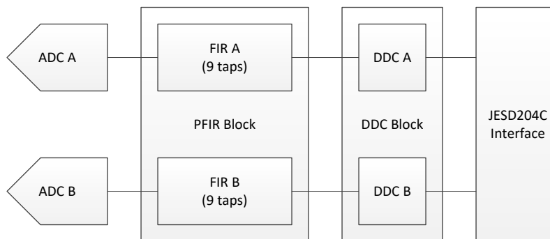
Figure 7. Dual Channel Equalization PFIR Block Diagram
