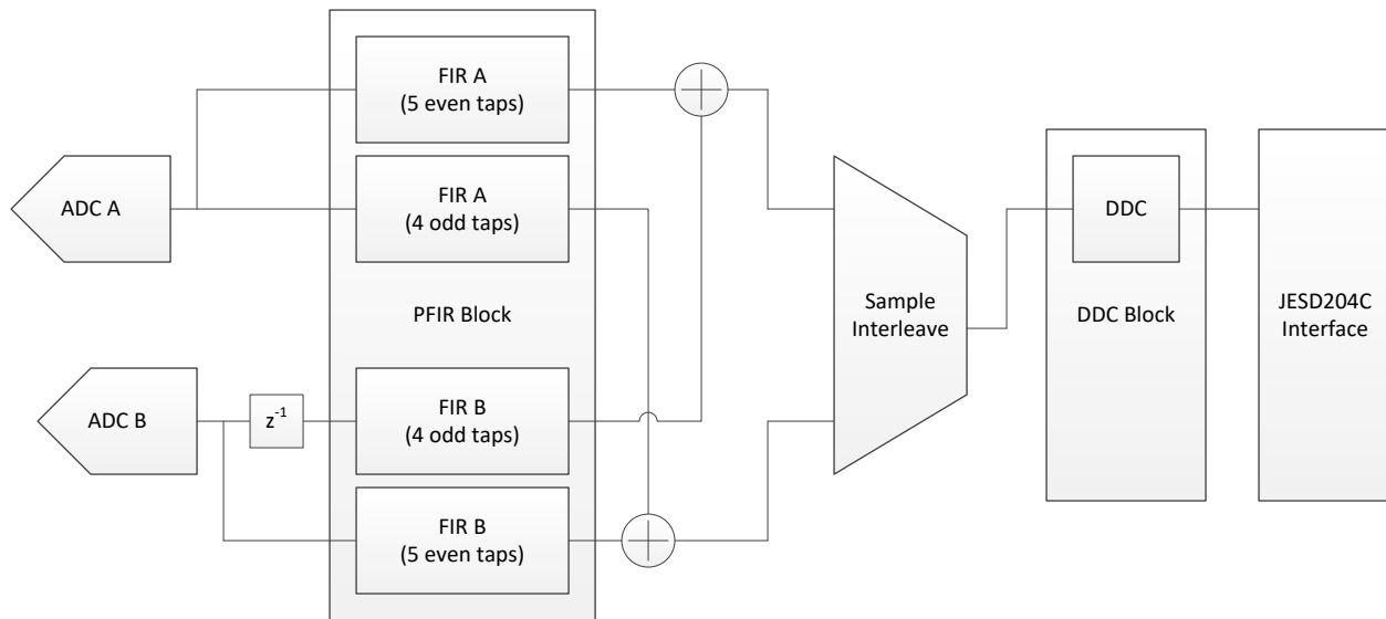
Figure 10. Alternate I/Q Correction-Type Filter Block Diagram
