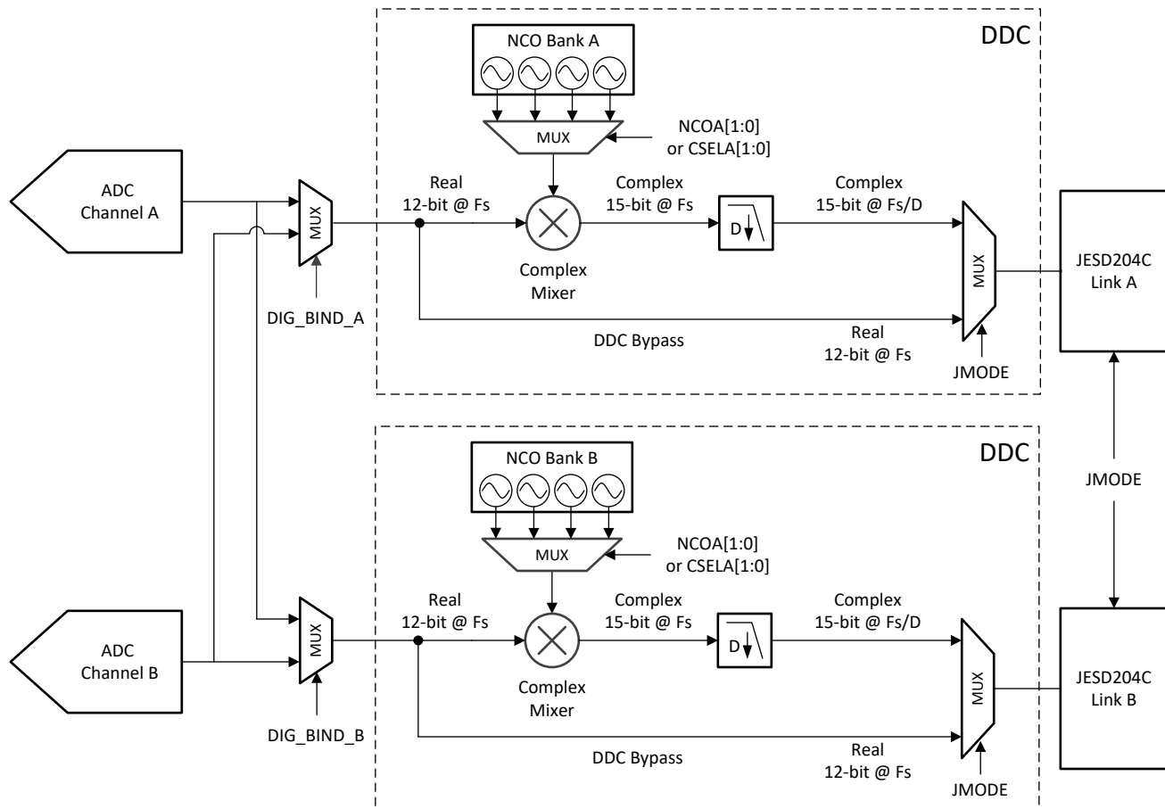
Figure 11. Digital Down Conversion Block in Dual Channel Mode
