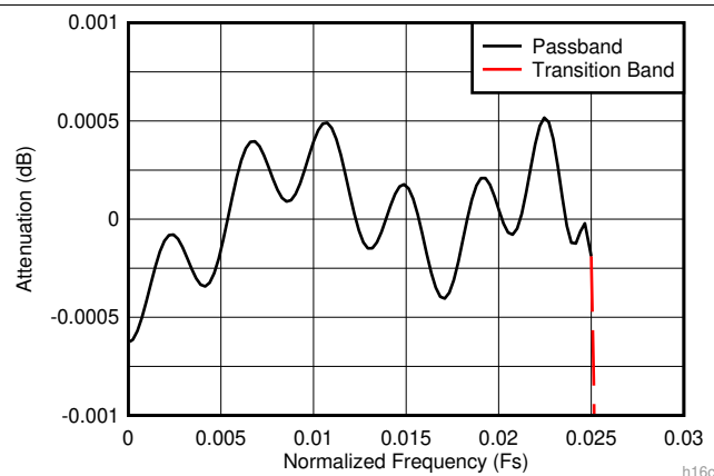
Figure 19. Decimate-by-16 Composite Zoomed Pass-Band Response
