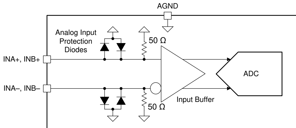
Figure 4. ADC12DJ5200RF Analog Input Internal Termination and Protection Diagram
