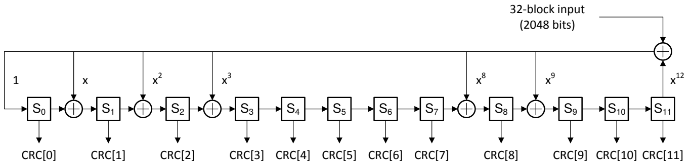
Figure 24. CRC-12 Parity Bit Generator
