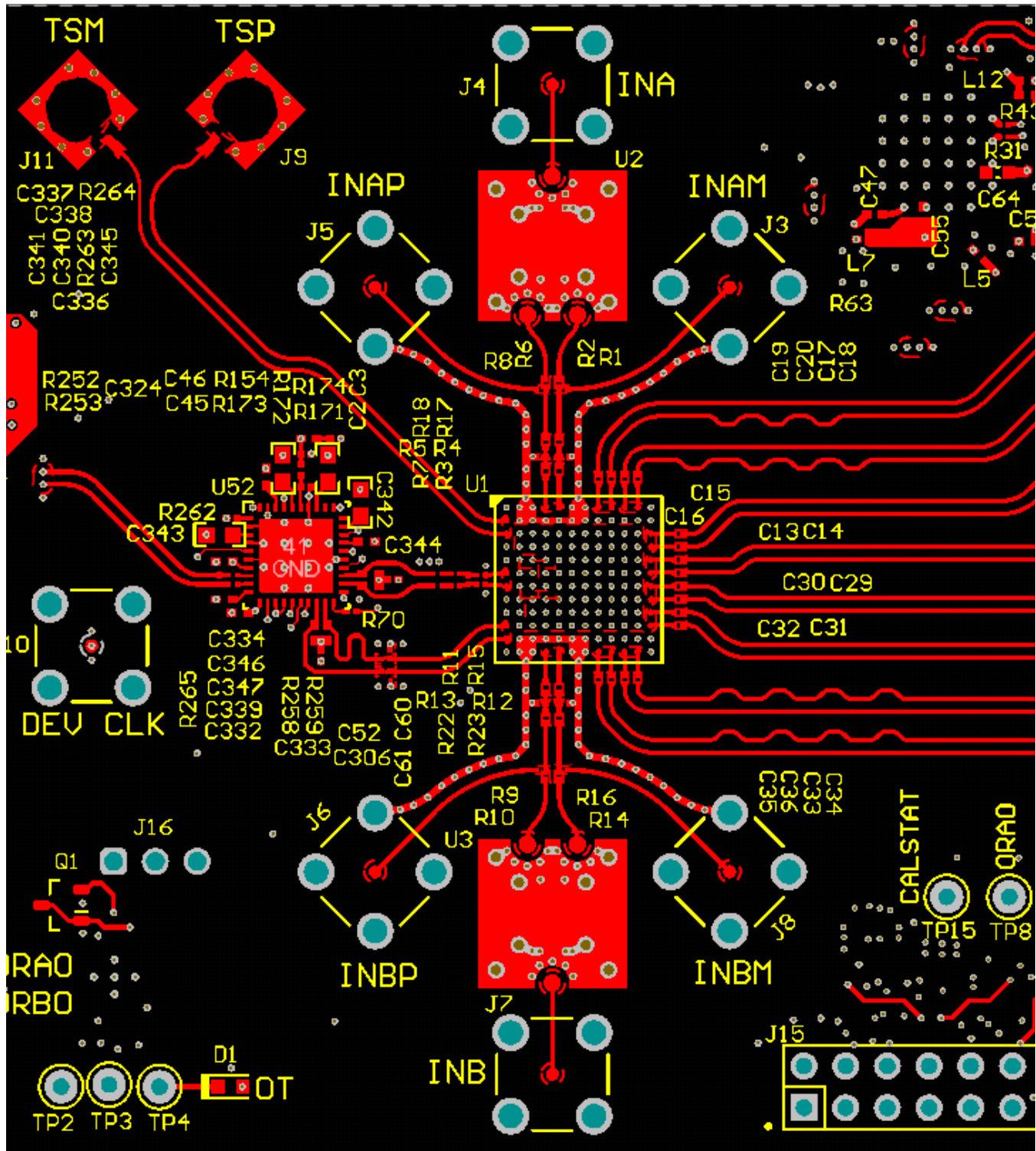
Figure 160. Top Layer Routing: Analog Inputs, CLK and SYSREF, DA0-3, DB0-3
