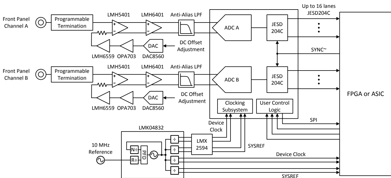
Figure 157. Typical Configuration for Reconfigurable Oscilloscope
