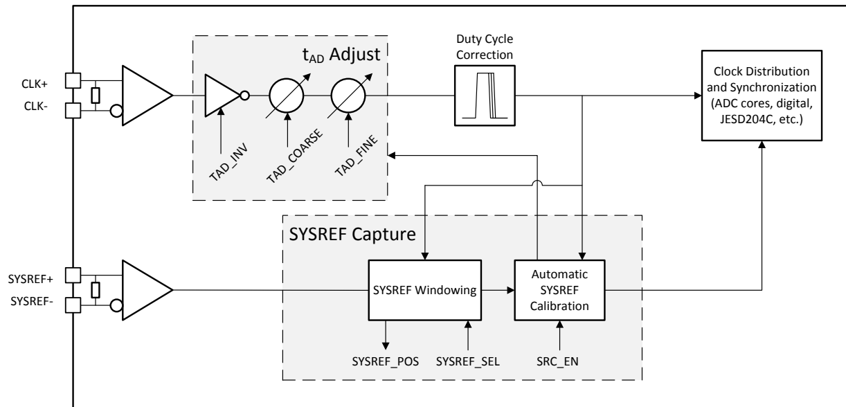
Figure 5. Clocking Subsystem
