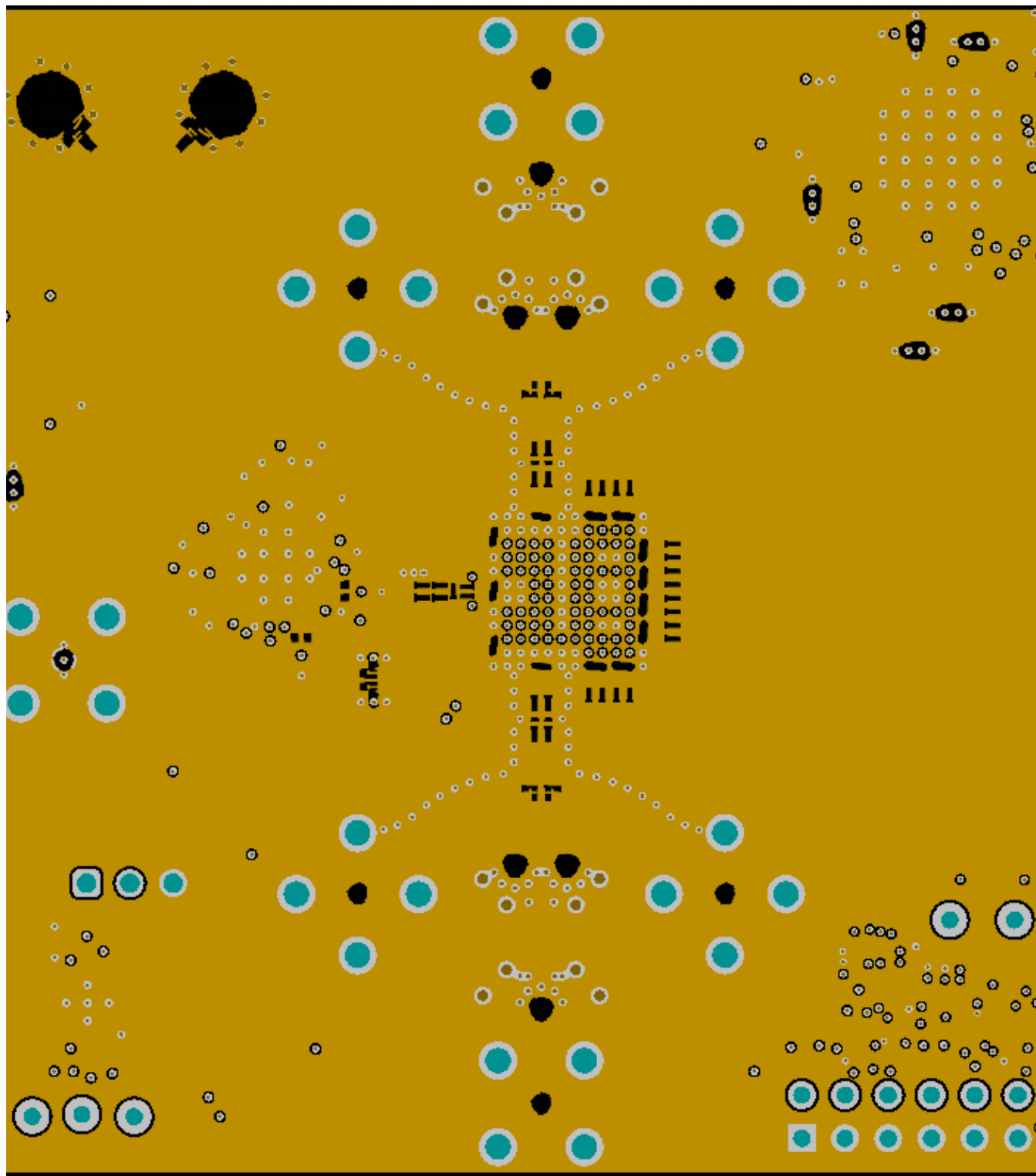
Figure 161. GND1 Cutouts to Optimize Impedance of Component Pads
