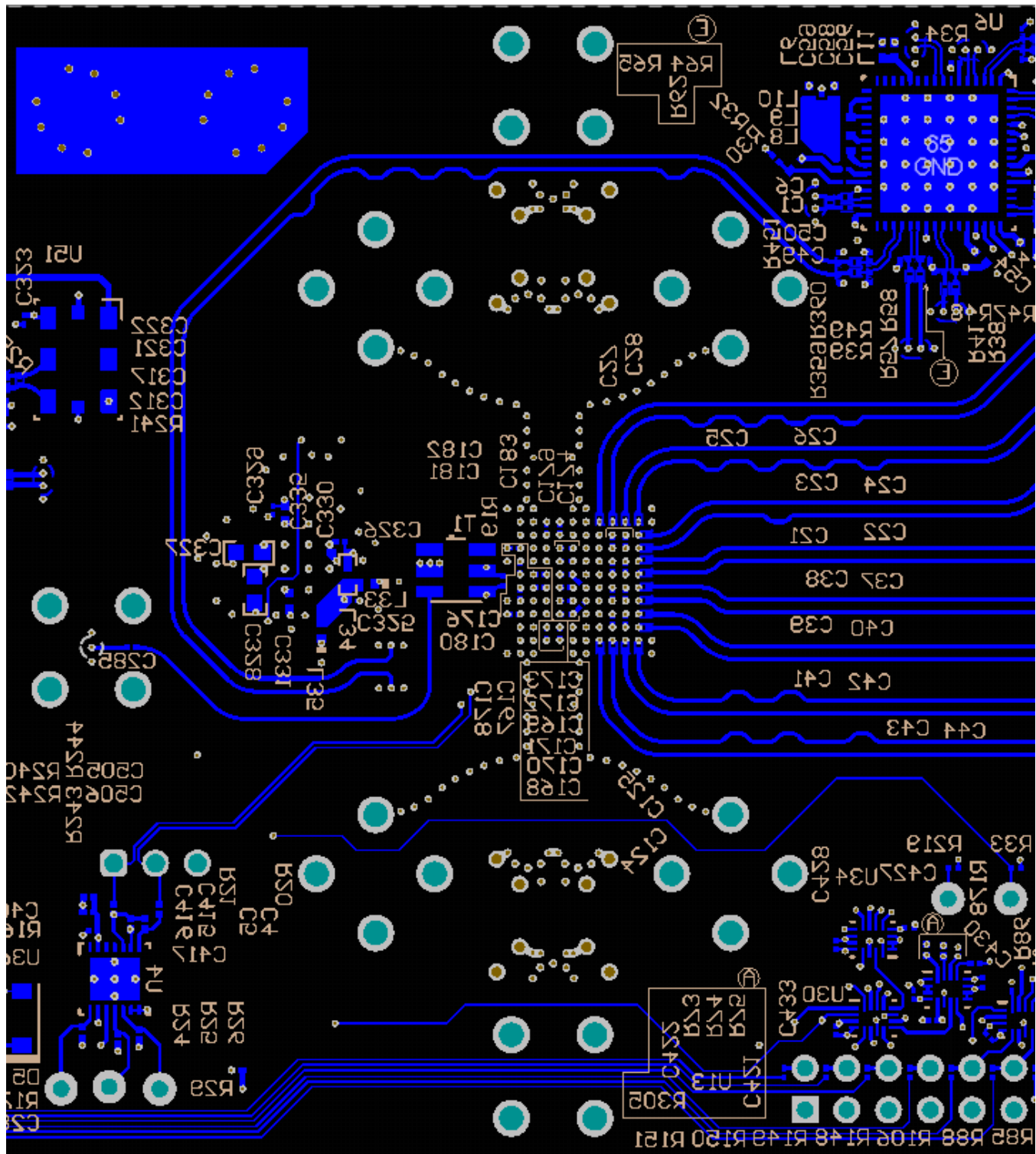
Figure 162. Bottom Layer Routing: Additional CLK Routing, DA4-7, DB4-7
