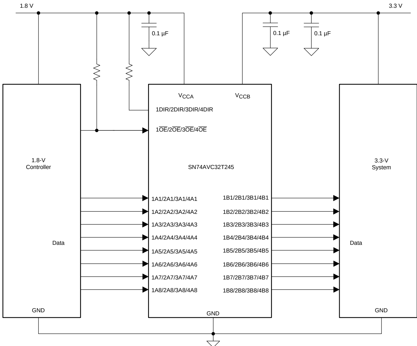
Figure 12. Application Schematic
