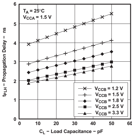
Figure 3. Typical Propagation Delay t_{PLH} (A to B) vs Load Capacitance
