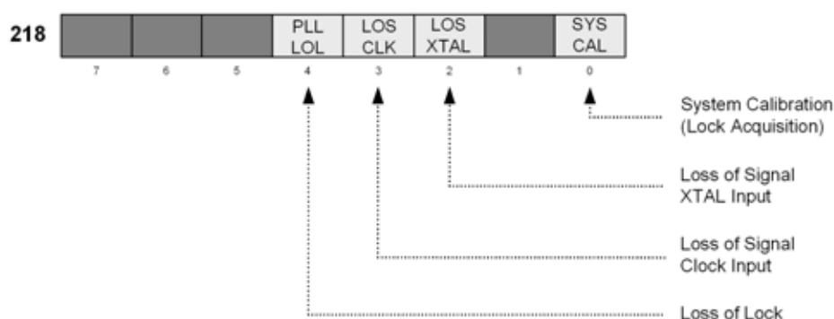
Figure 5. Status Register
