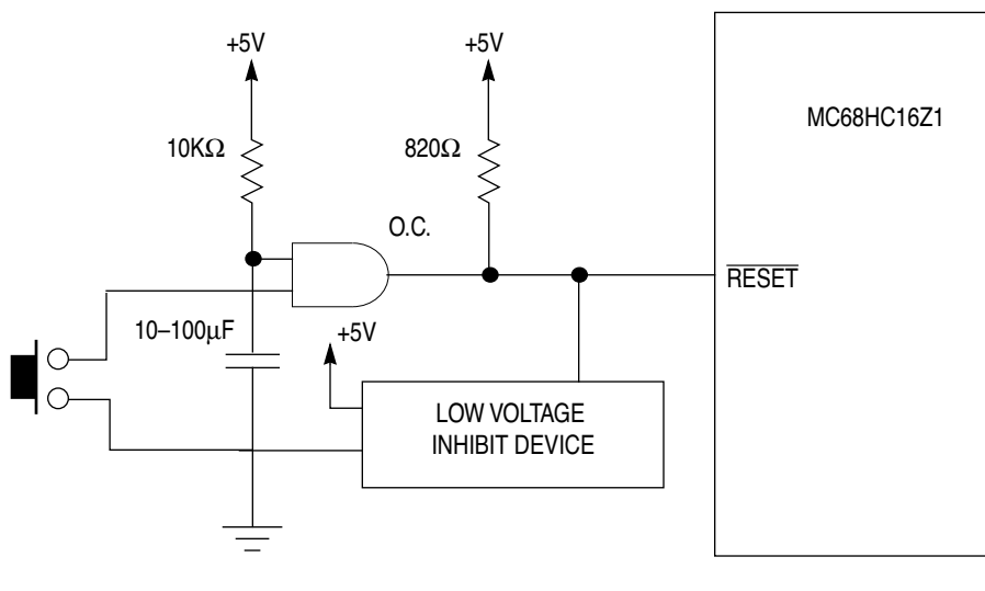
Figure 7 Typical MC68HC16Z1 Reset Circuit
