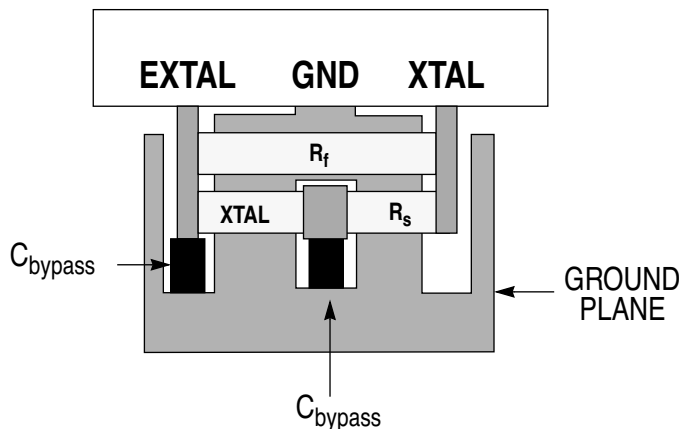
Figure 5 Typical One-Layer Oscillator Layout
