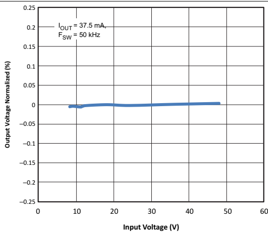
Figure 45. Output Voltage Normalized vs Input Voltage
