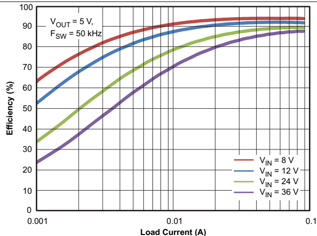
Figure 40. Efficiency vs Load Current
