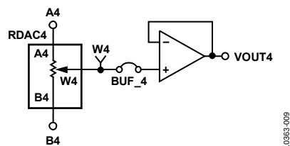
Figure 9. RDAC4
