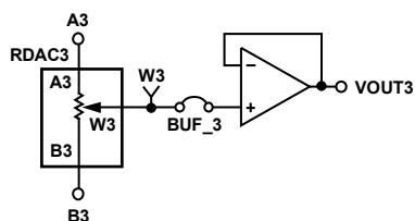
Figure 8. RDAC3
