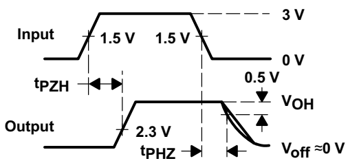
VOLTAGE WAVEFORMS
