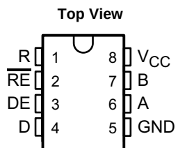
Pin Functions
