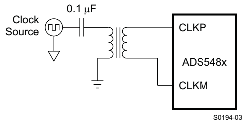
Figure 71. Differential Clock
