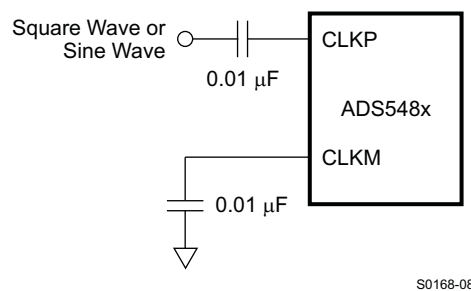
Figure 68. Single-Ended Clock
