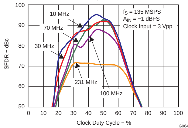
Figure 74. SFDR vs Clock Duty Cycle
