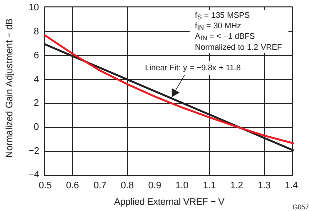
Figure 62. Signal Gain Adjustment versus External Reference (VREF)
