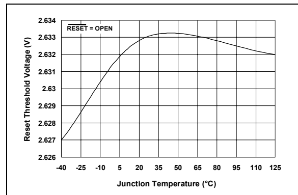
FIGURE 2-29: Reset Threshold Voltage vs. Junction Temperature.
