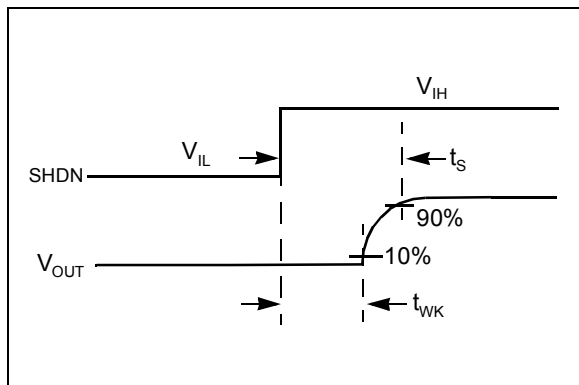
FIGURE 4-1: Wake-up From \overline{\text{SHDN}} .
