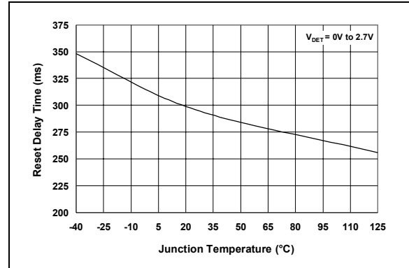
FIGURE 2-28: Power-Up Reset Time-out Period vs. Junction Temperature.
