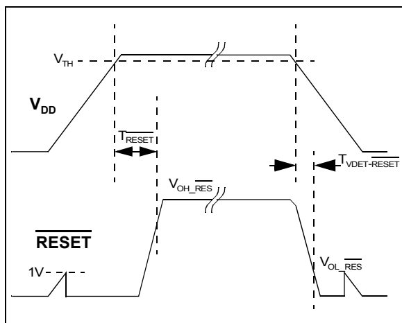
FIGURE 4-2: \overline{\text{RESET}} Timing Diagram.
