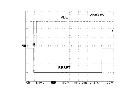
FIGURE 2-35: Power-Up RESET Timing.
