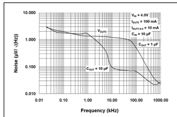
FIGURE 2-24: Output Noise.
