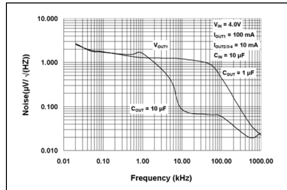
FIGURE 2-23: Output Noise.
