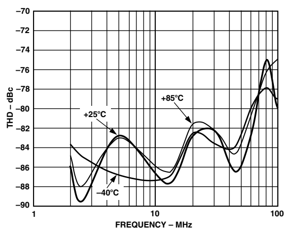
TPC 12. THD vs. Temperature and Frequency
