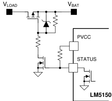
Figure 18. Disconnection Switch Control Example
