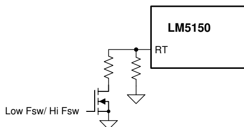
Figure 25. Dynamic Frequency Change
