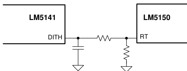
Figure 23. Dithering Using Dither Enabled Device LM5141
