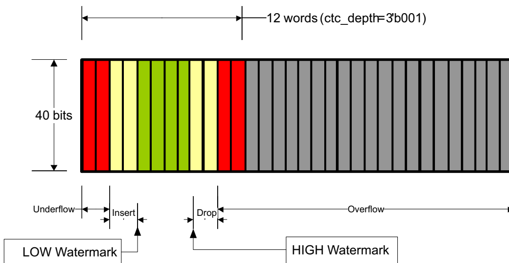
Figure 5-29. Organization of the XAUI CTC FIFO (12-Deep)
