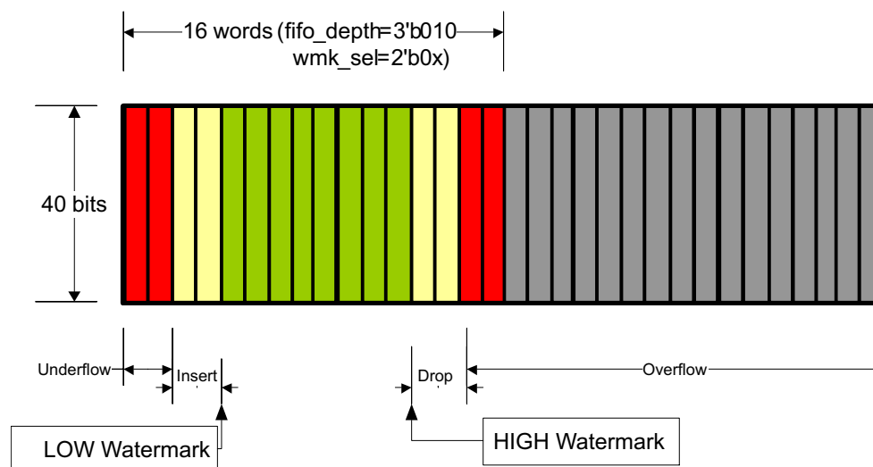
Figure 5-27. Organization of the XAUI CTC FIFO (16-Deep, Low Watermark)
