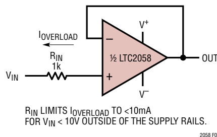
Figure 9. Using a Resistor to Limit Input Current
