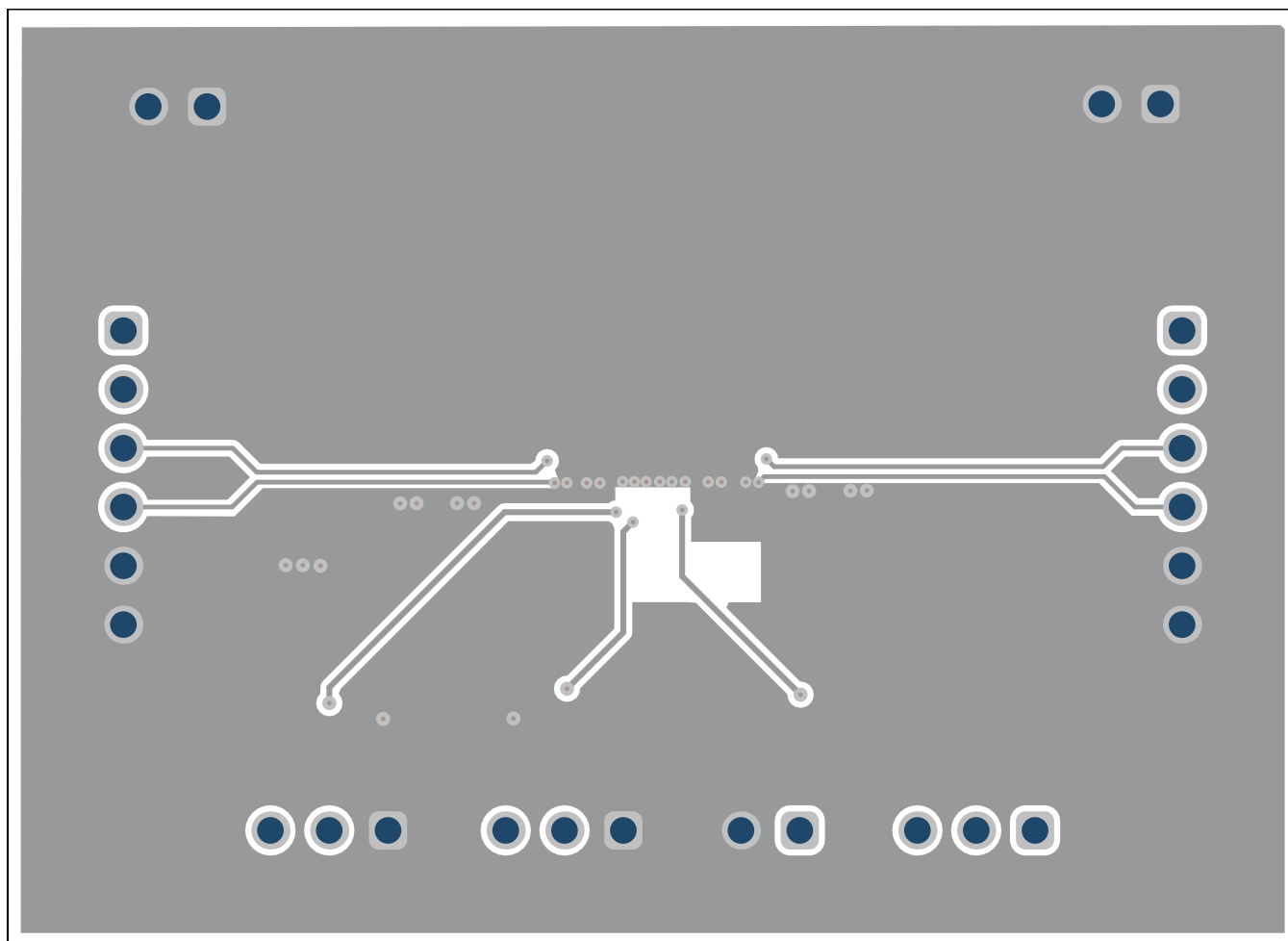
Figure 4. Signal Layer 2
