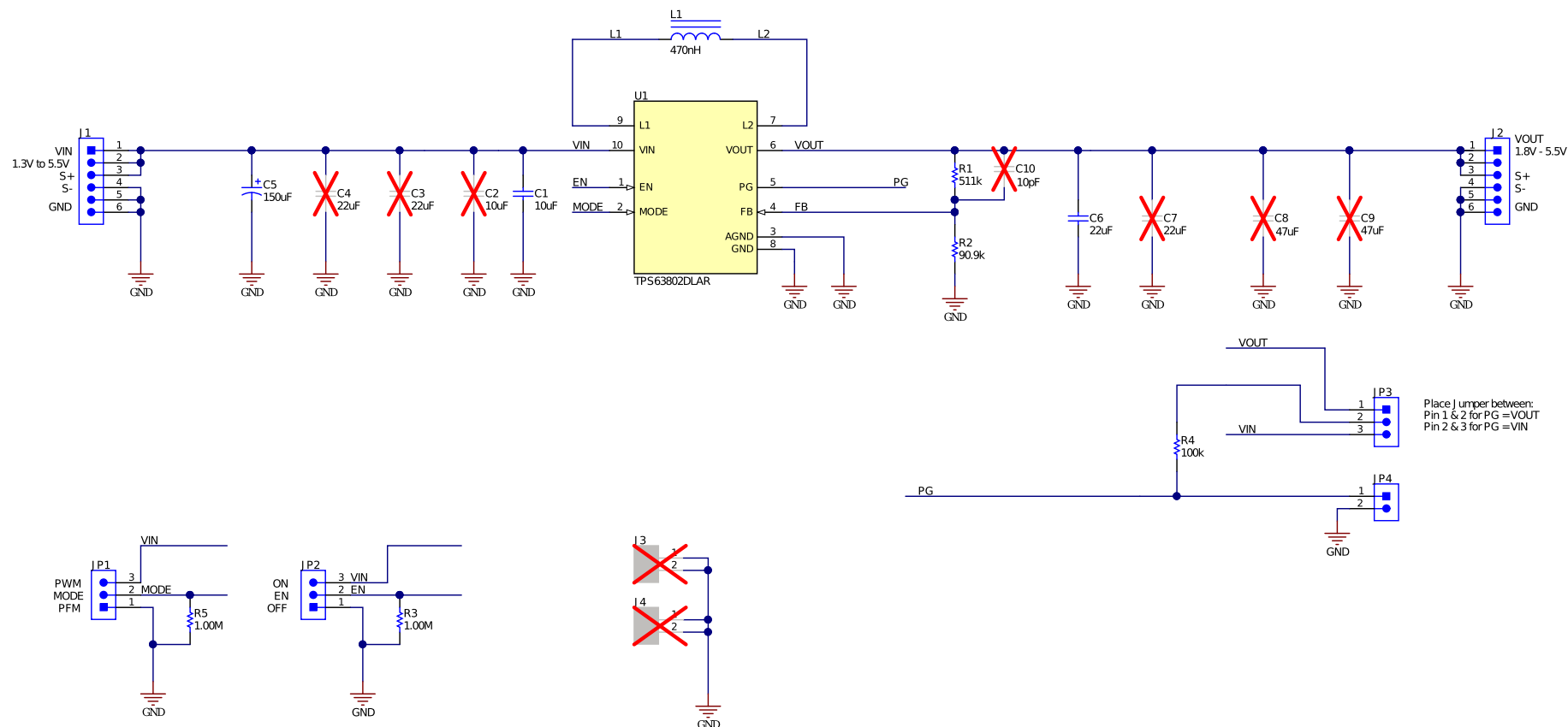
Figure 6. Schematic
