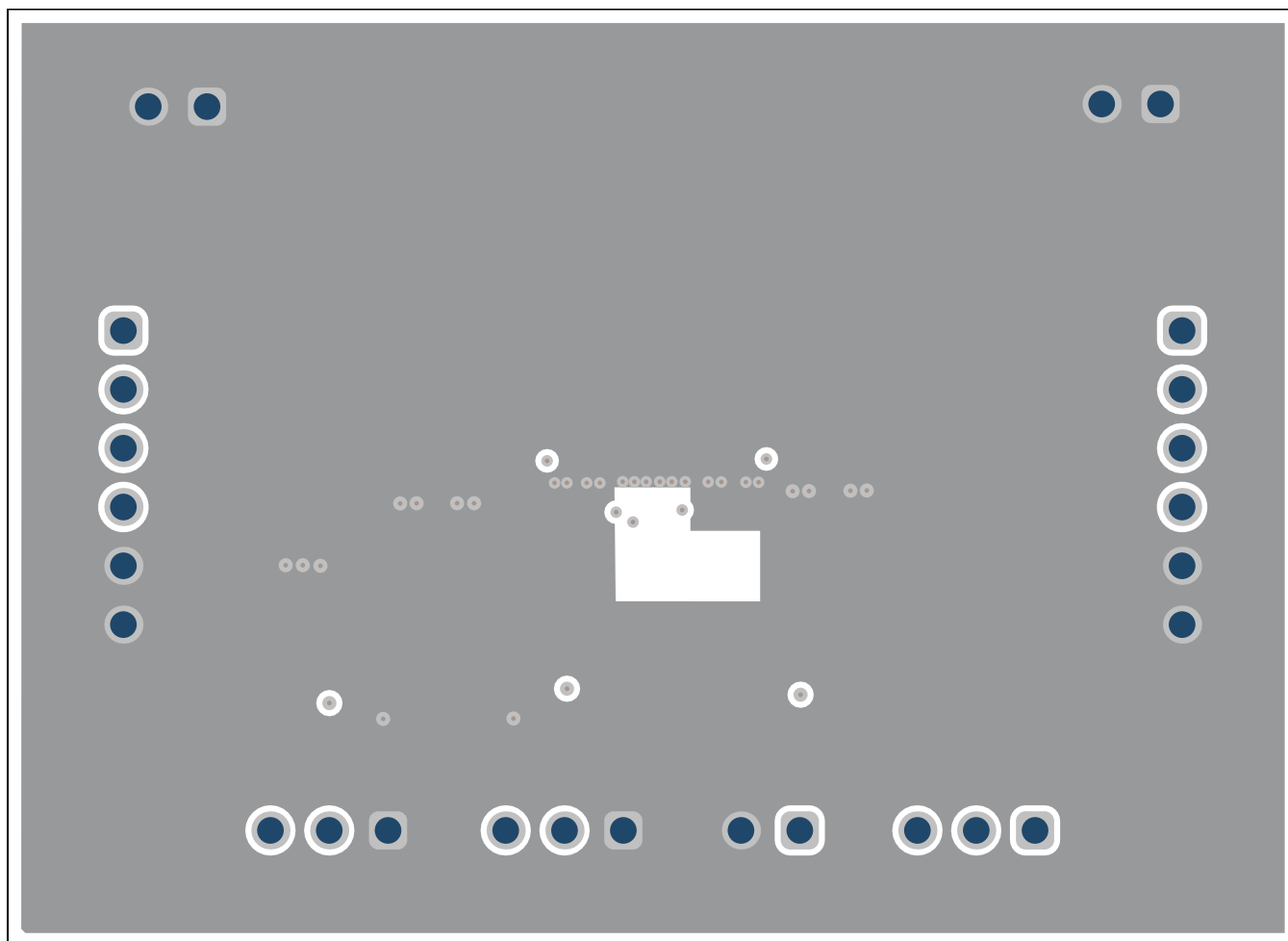
Figure 3. Signal layer 1
