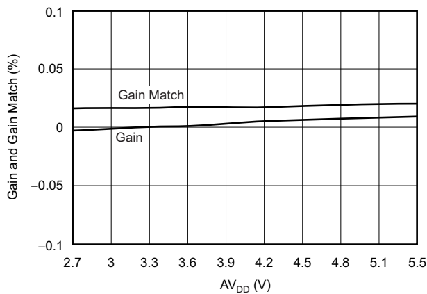
Figure 12. GAIN ERROR AND GAIN MATCH vs ANALOG SUPPLY VOLTAGE
