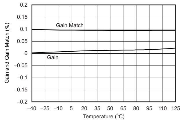
Figure 13. GAIN ERROR AND GAIN MATCH vs TEMPERATURE
