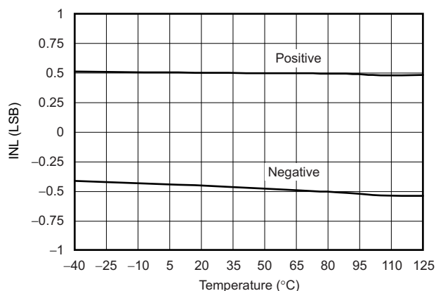
Figure 5. INTEGRAL NONLINEARITY vs TEMPERATURE
