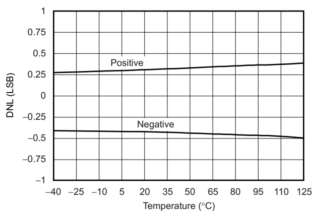
Figure 9. DIFFERENTIAL NONLINEARITY vs TEMPERATURE
