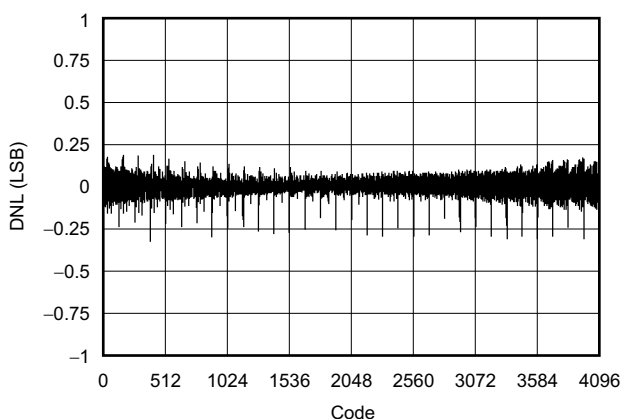
Figure 7. DIFFERENTIAL NONLINEARITY vs CODE
