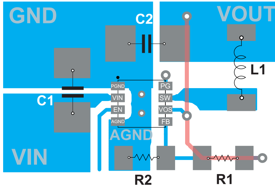
Figure 38. Layout Example
