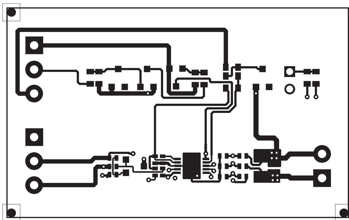
Figure 4. bq27200EVM Layer 1 Layout
