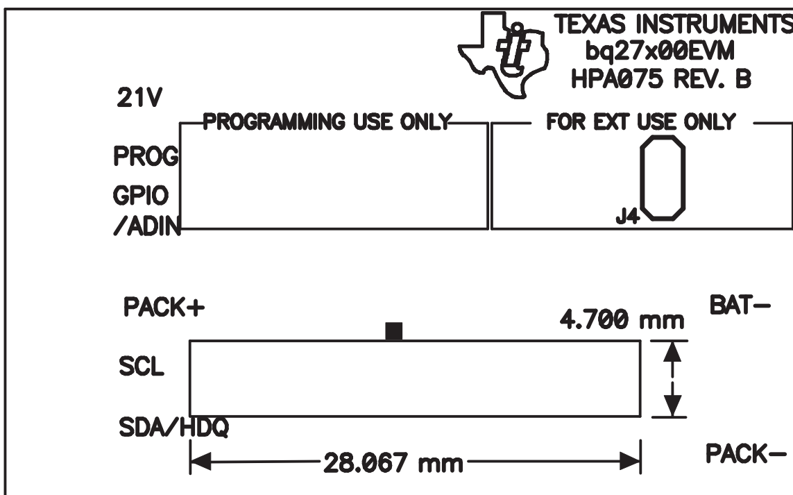
Figure 3. bq27200EVM Silkscreen
