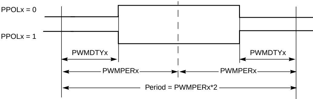
Figure 12-38. PWM Center Aligned Output Waveform
