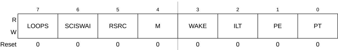
Figure 8-5. SCI Control Register 1 (SCICR1)
