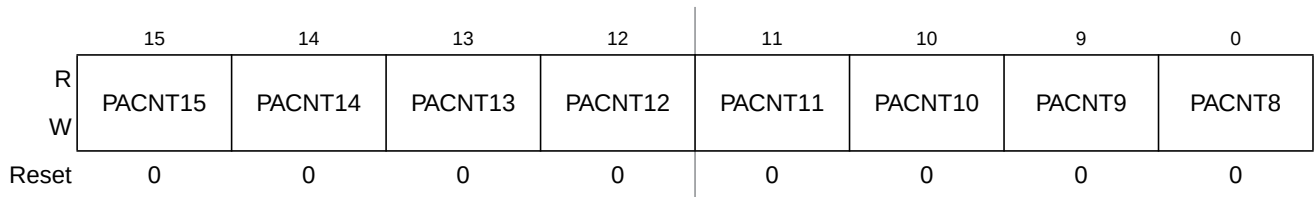
Figure 13-24. Pulse Accumulator Count Register High (PACNTH)
