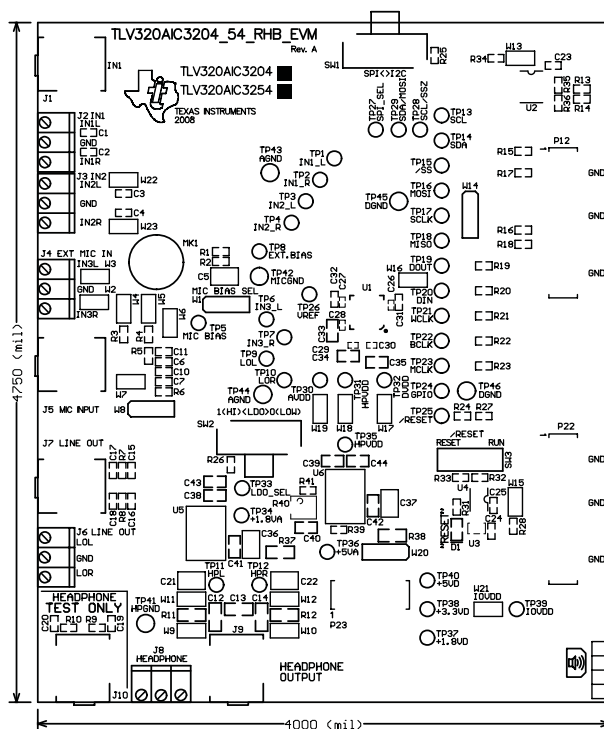
Figure 24. Top Overlay
