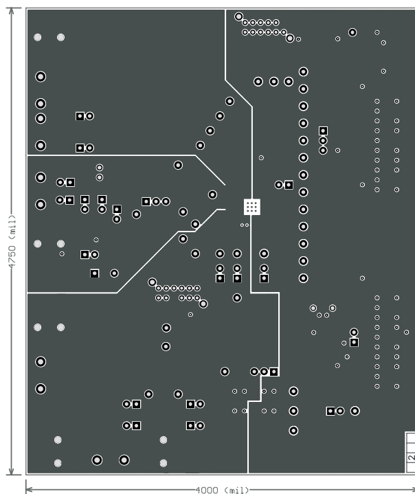
Figure 21. Mid-Layer 1
