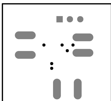
Figure 32. Bottom Silkscreen
