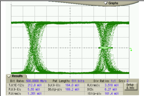
FIGURE B-5: 30M CAT6 CABLE AFTER EQUALIZER
