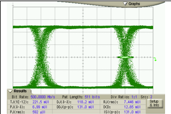
FIGURE B-6: 60M CAT6 CABLE AFTER EQUALIZER
