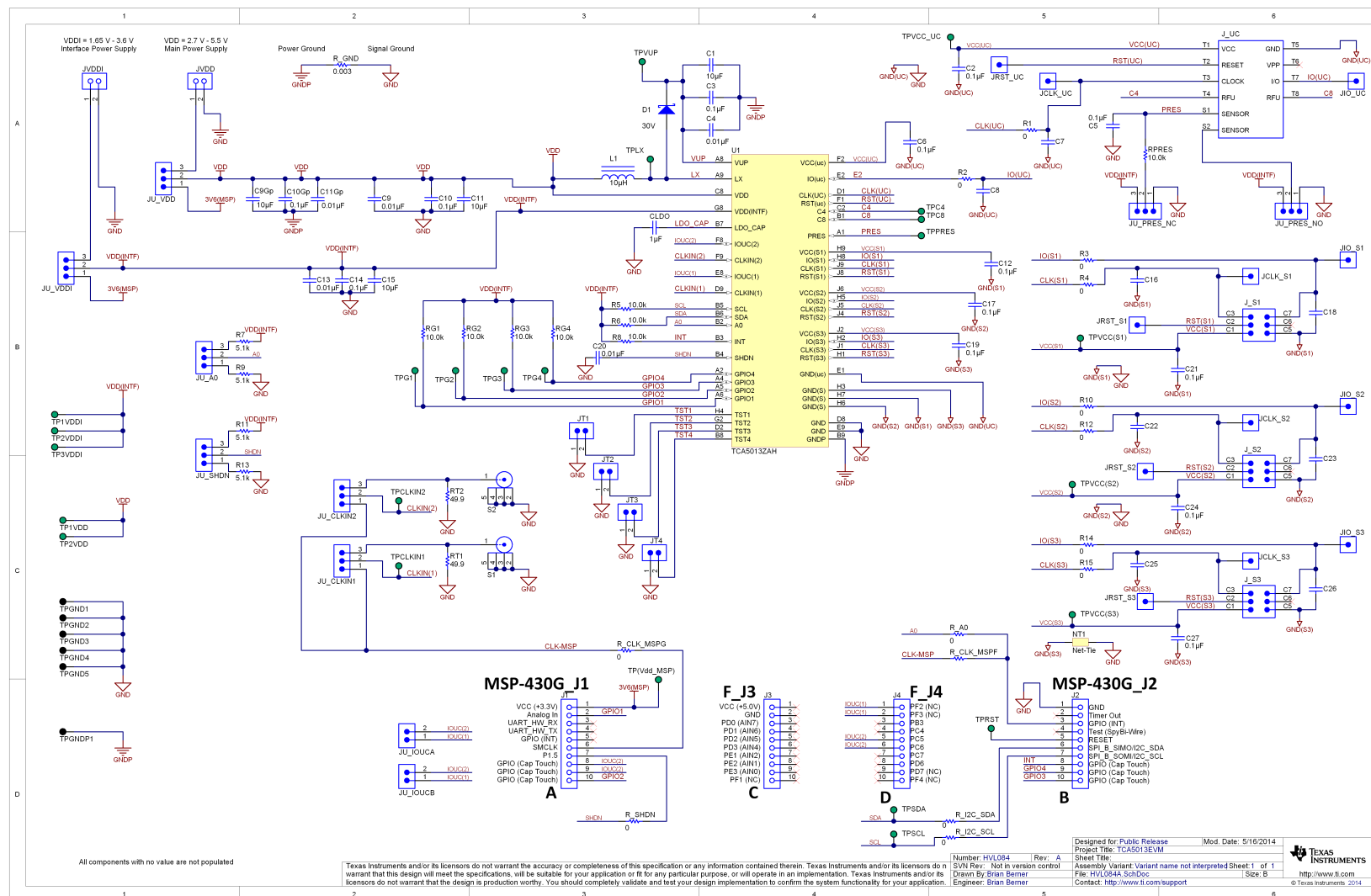
Figure 2. TCA5013EVM Schematic
