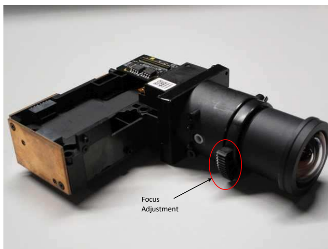
Figure 6-1. Optical Engine with Focus Adjustment
