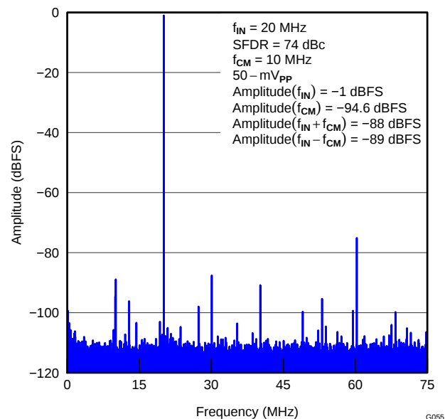
Figure 35. COMMON-MODE REJECTION RATIO SPECTRUM FOR AVDD SUPPLY
