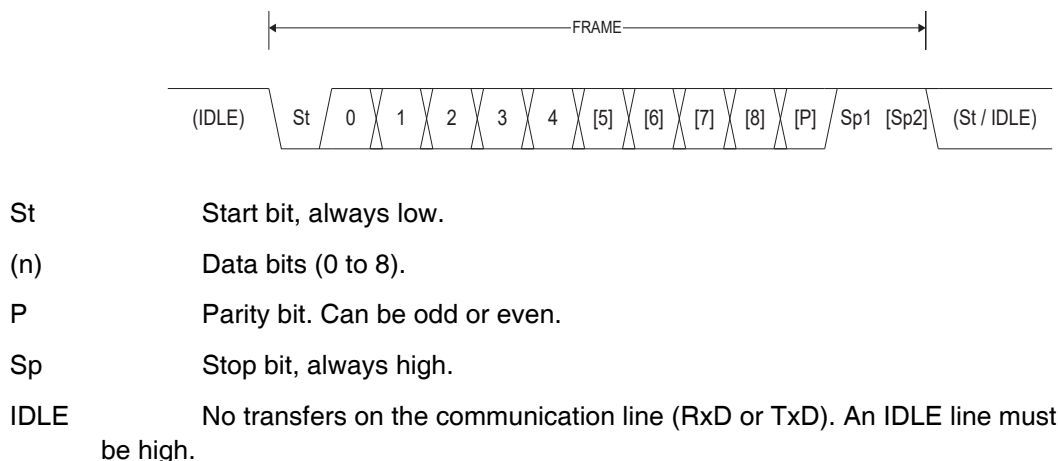
Figure 20-4. Frame Formats
