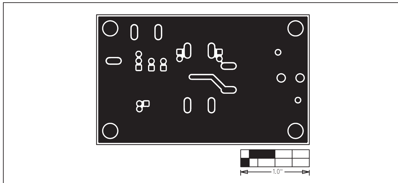
Figure 4. MAX4993 EV Kit PCB Layout—Solder Side
