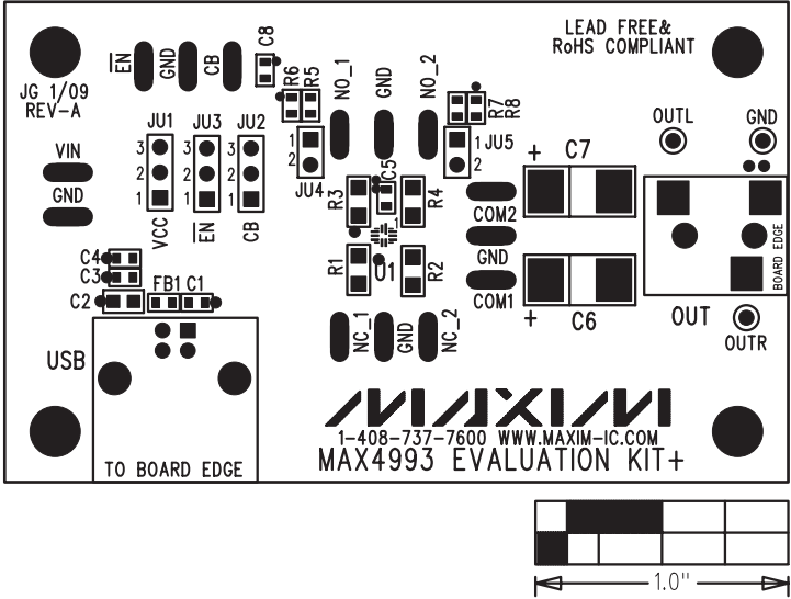
Figure 2. MAX4993 EV Kit Component Placement Guide—Component Side
