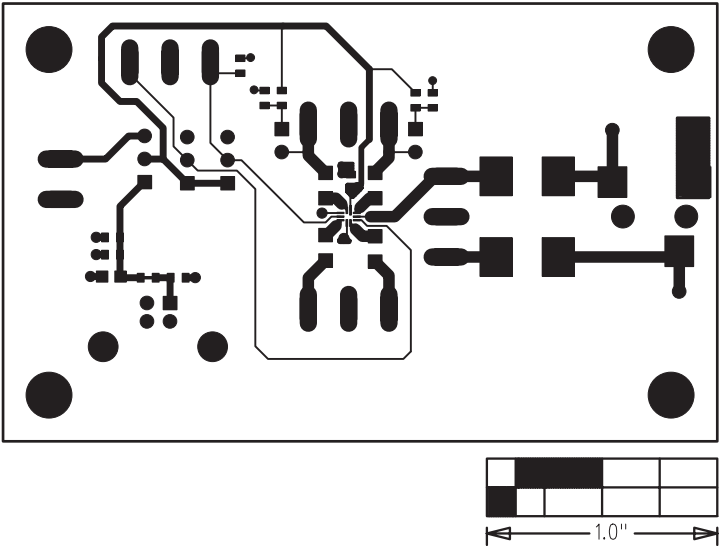
Figure 3. MAX4993 EV Kit PCB Layout—Component Side
