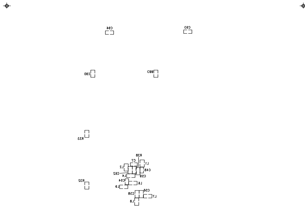
Figure 23. EVAL-AD7763EDZ Solder Side Layer 4 Artwork
