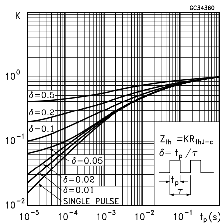
Figure 5. Thermal impedance for TO-220
