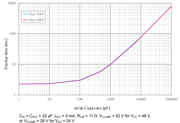
Figure 9. Startup time vs. C_{dv/dt}
