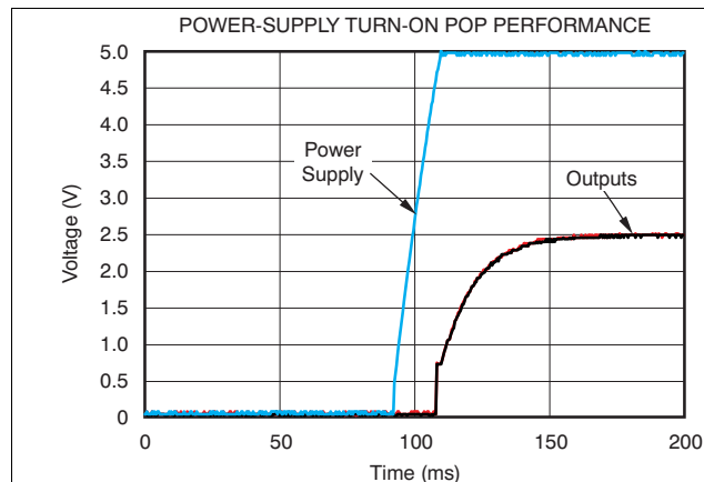
Figure 70. THS4521 Power-Supply Turn-On Pop Performance
