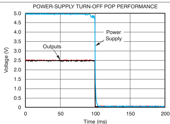
Figure 71. THS4521 Power-Supply Turn-Off Pop Performance
