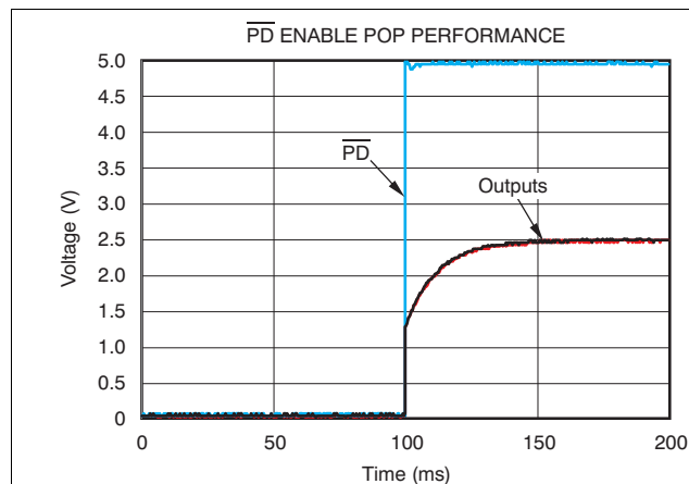
Figure 72. THS4521 \overline{\text{PD}} Pin Enable Pop Performance
