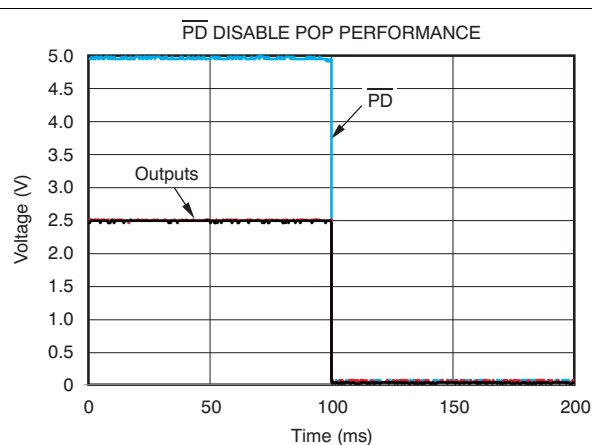
Figure 73. THS4521 \overline{\text{PD}} Pin Disable Pop Performance
