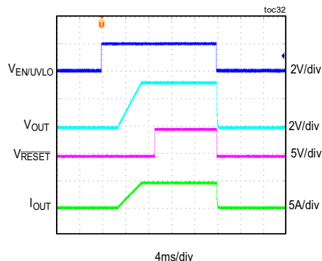
POWER-UP WITH 2.5V BIAS
