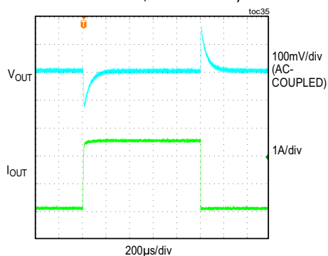
LOAD TRANSIENT
