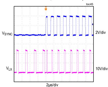
SYNC FREQUENCY AT 630kHz ( V_{IN} = 24V , V_{OUT} = 5V , I_{OUT} = 5A PWM MODE, MODE = SGND)
