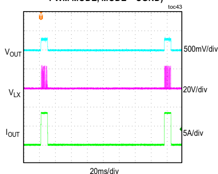
OUTPUT SHORT IN STEADY STATE ( V_{IN} = 24V , V_{OUT} = 5V , OUTPUT SHORT PWM MODE, MODE = SGND)
