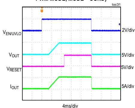
POWER-UP WITH 2.5V BIAS
