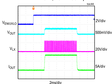
STARTUP INTO SHORT ( V_{IN} = 24V , V_{OUT} = 5V , OUTPUT SHORT PWM MODE, MODE = SGND)
