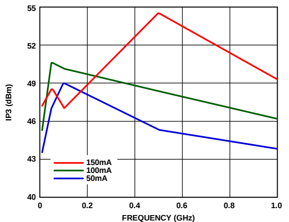
Figure 19. Output Third-Order Intercept ( IP_3 ) vs. Frequency at Various Supply Currents, P_{OUT}/Tone = 30\text{ dB}
