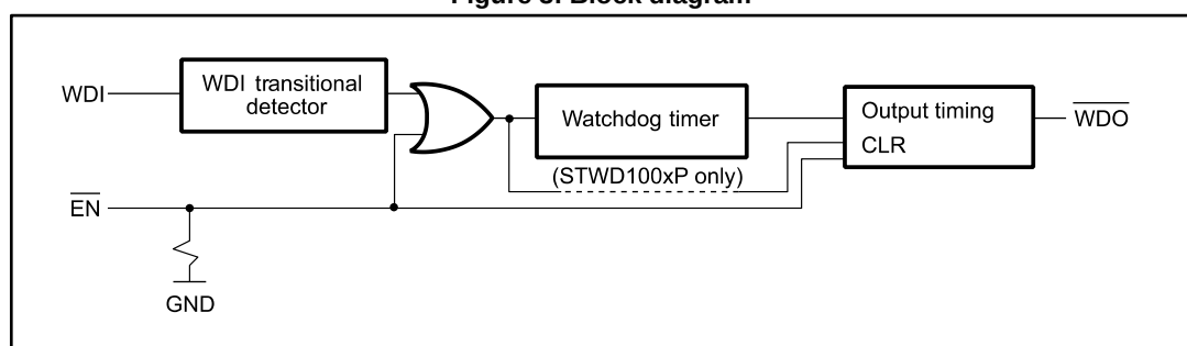
Figure 3: Block diagram
